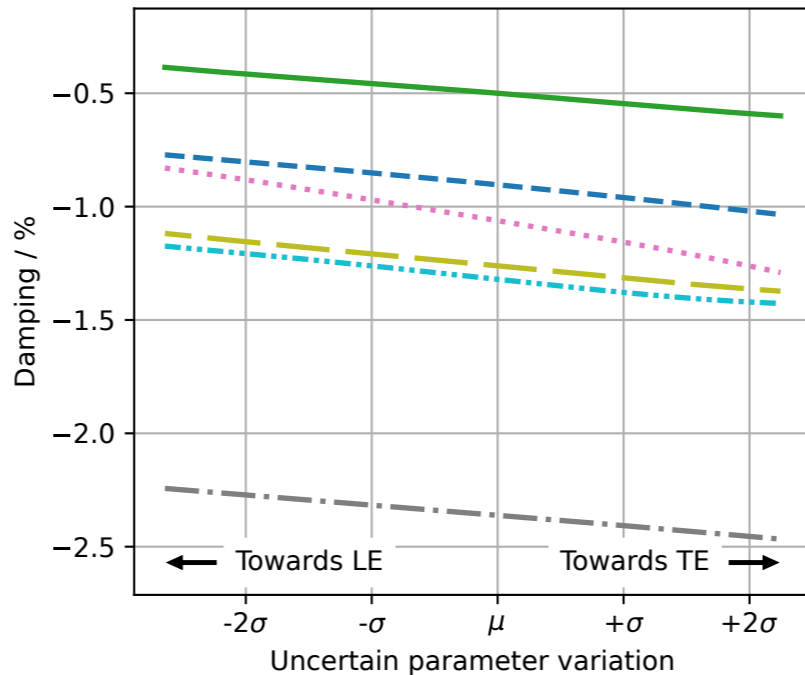
Chordwise COG
