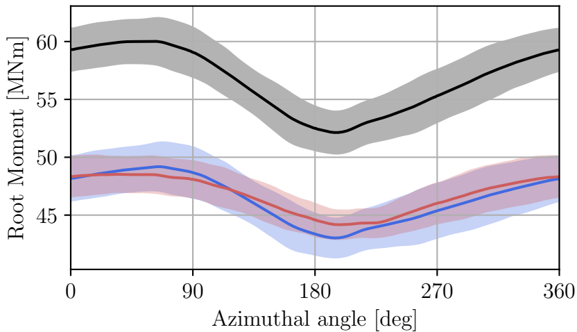
Flapwise M_z
