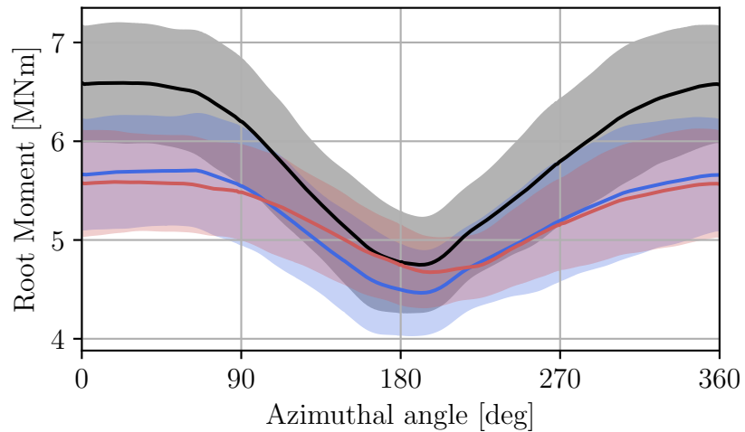
Edgewise M_x
