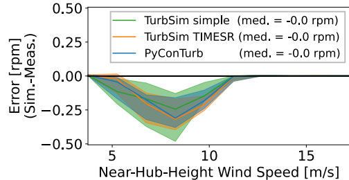
(a) Rotor Speed Mean
