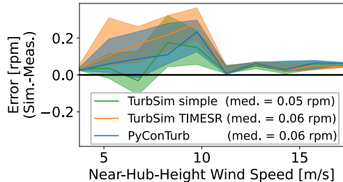
(a) Rotor Speed Standard Deviation
