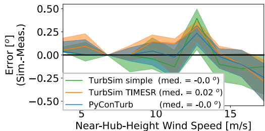
(b) Blade Pitch Standard Deviation, Blade 2
