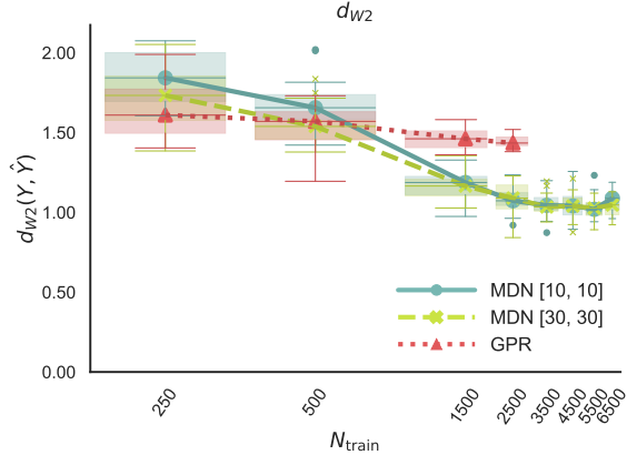
(b) d_{W_2}(Y, \hat{Y})
