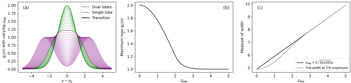
Figure A1. (a) Double Gaussian curves, g_2(x) , with varying z_{\text{sep}} and fixed amplitude a = 1 and width \sigma = 1 showing the transition of classification from near-wake (purple) to far-wake (green) fits using an empirically picked threshold of z_{\text{sep}} = 2\sigma (black). The corresponding (b) maximum and (c) width of the double Gaussian as a function of z_{\text{sep}} .
