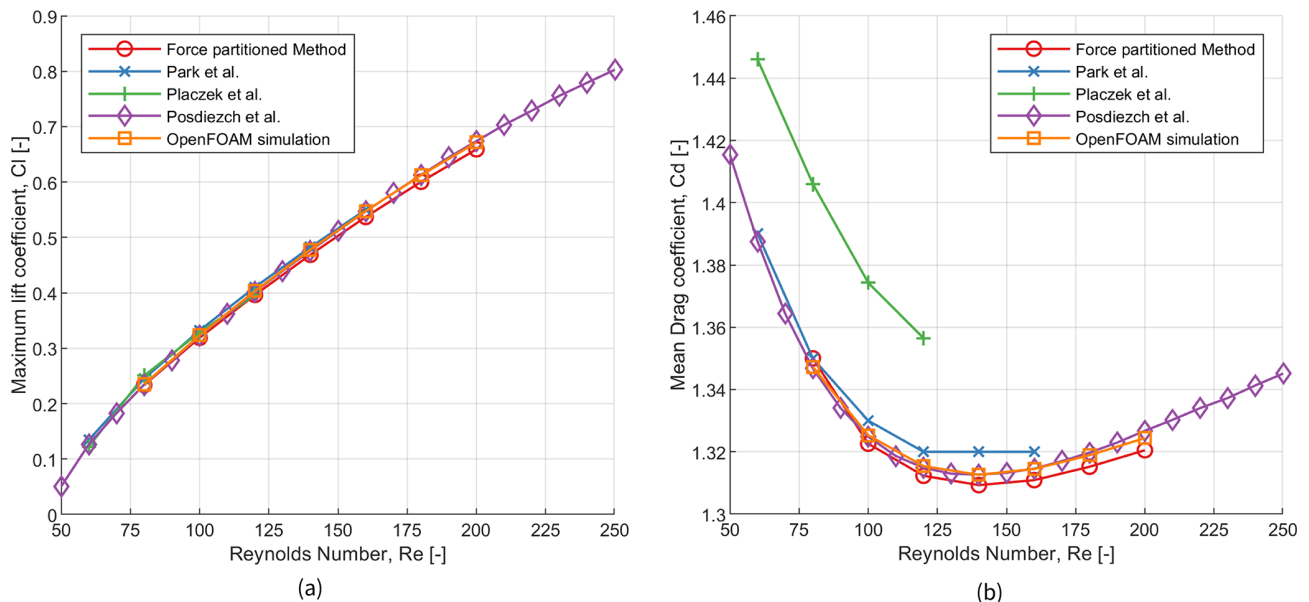
Figure 7. Variation in (a) maximum lift coefficient and (b) mean drag coefficient for a fixed cylinder at different subcritical Reynolds numbers compared against the literature: Park et al. (1998), Placzek et al. (2009), and Posdziech and Grundmann (2007).
