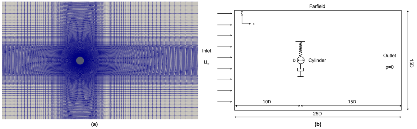
Figure 4. Schematic representation of the computational domain: computational mesh (a), domain characteristics (b).
