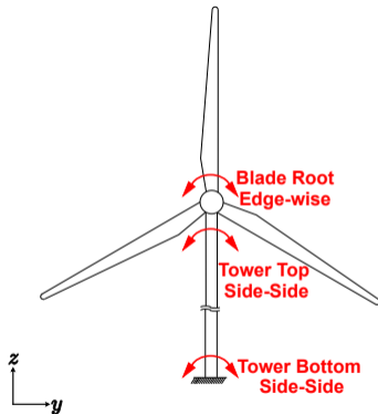
(b) OpenFAST output channels y, z plane
