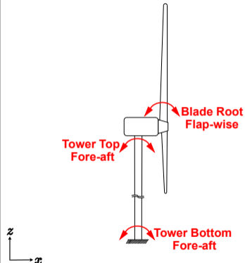
(c) OpenFAST output channels x, z plane
