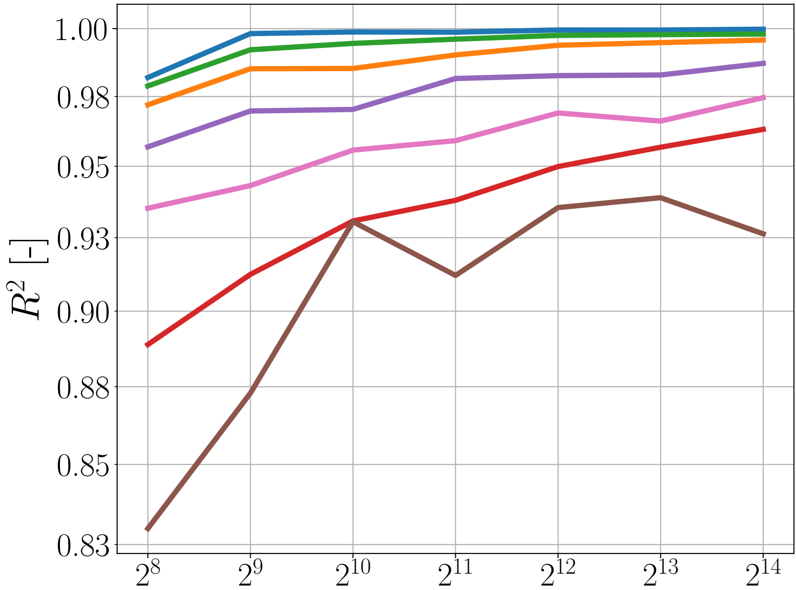
TCN-FCNN
