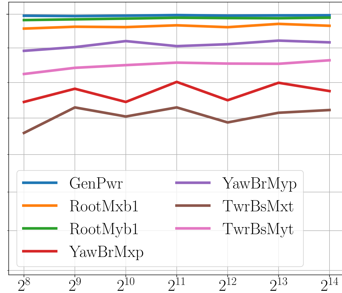
FCNN
