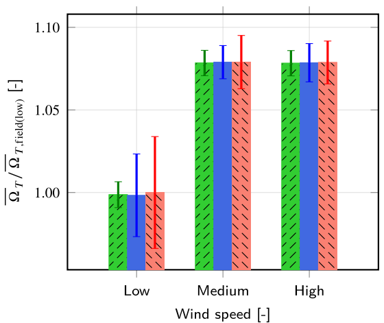
(b) Rotation speed
