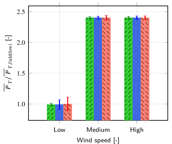
(c) Power output
