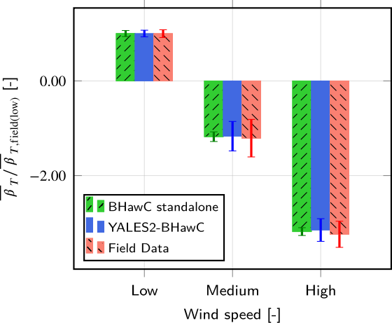
(a) Total pitch angle (blade 1)
