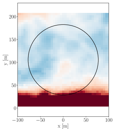
(e) Medium speed - YALES2 ( z = -2D )
