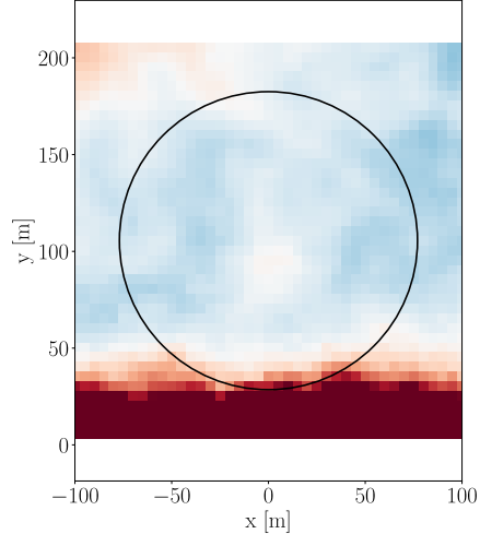
(b) High speed - YALES2 ( z = -2D )
