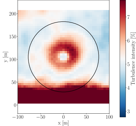
(c) High speed - YALES2 ( z = 0 )
