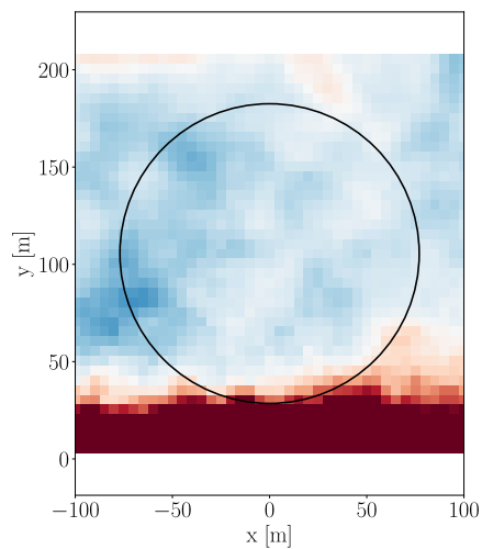
(h) Low speed - YALES2 ( z = -2D )
