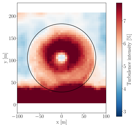
(f) Medium speed - YALES2 ( z = 0 )
