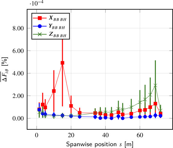
(a) Internal forces
