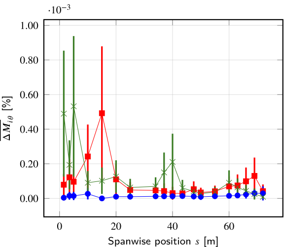
(b) Internal moments
