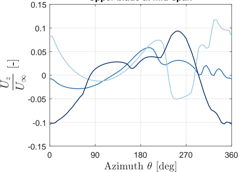
Upper blade at mid-span
