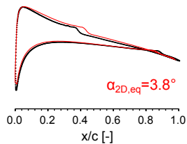
(c) 90% span
