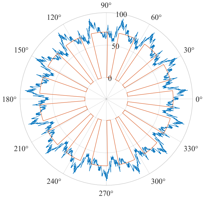
Resulting load cycles on inner ring
