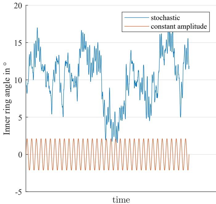
Bearing movement
