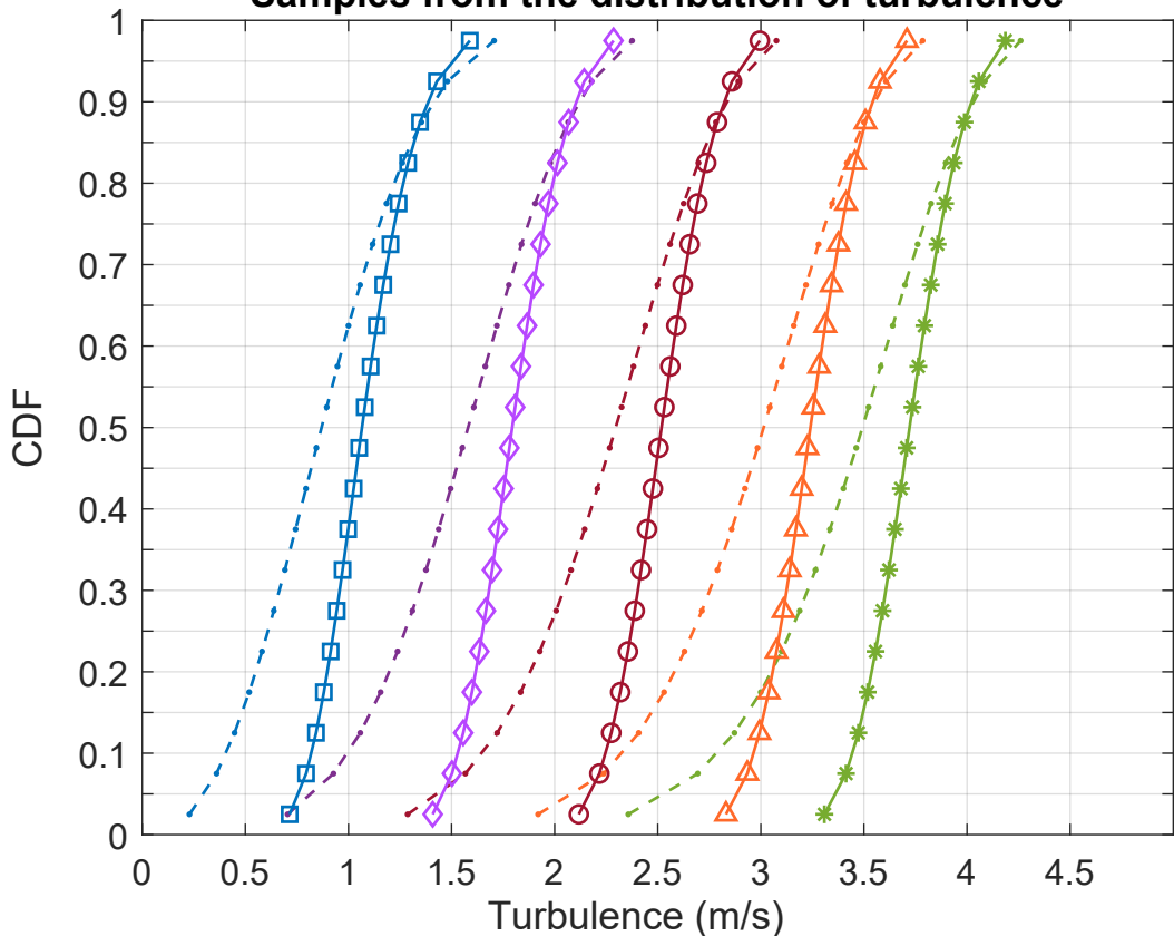
Samples from the distribution of turbulence
