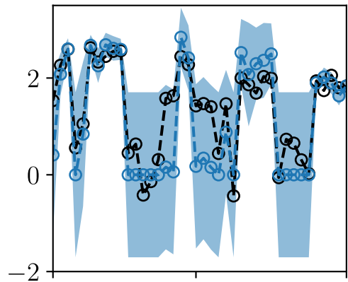
RBF
