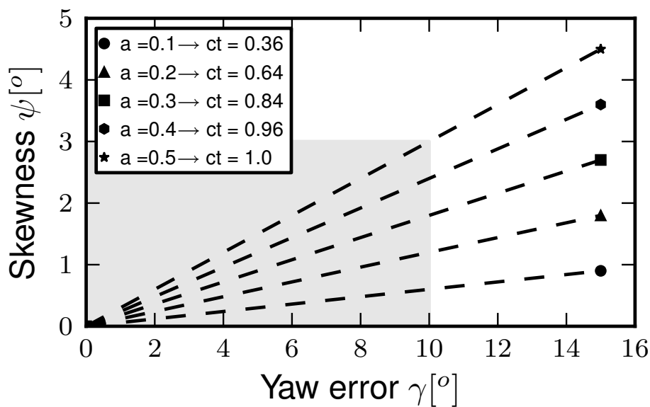
Fig. 1. Approximated theoretical expectation of the effect of wind turbine misalignment on wake skewness with respect to induction (a) or thrust coefficient (Ct)
