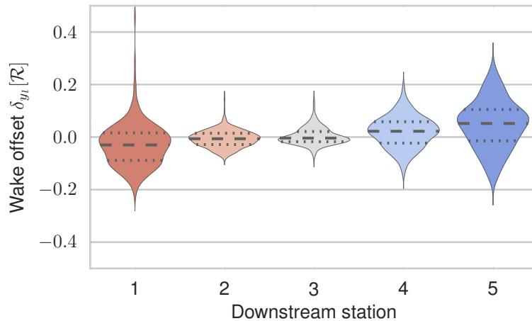
Figure 7. Violin plot of statistics showing the distribution of the frequency of the horizontal wake offset. The dashed lines represent the 25th, 50th and 75th percentile. \delta_{y_i} is given in rotor radius [R].
