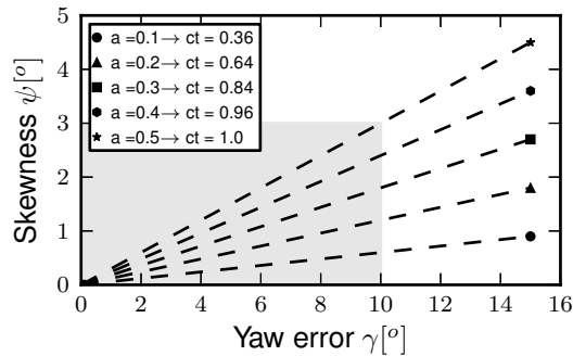
Figure 11. Representation of the effect of wind turbine misalignment ( \gamma ) on wake skewness ( \psi ).
