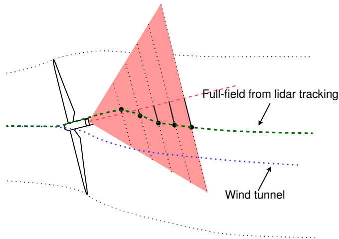
Figure 9. Sketch of our interpretation of the measured near wake path for an individual yaw misalignment; showing what we call a delay shift with respect to wind tunnel paths found in publications.
