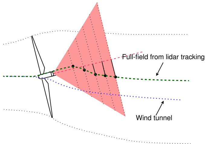
Figure 9. Sketch of our interpretation of the measured near wake path for an individual yaw misalignment; showing what we call a deviation shift with respect to wind tunnel paths found in publications.
