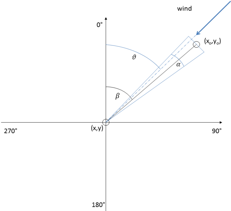
5 Figure 3: Determination of free flow turbines for wind speed averaging. The turbine at (x_0,y_0) produces a wake on the turbine at (x,y) for the displayed wind direction \vartheta . \beta is the angle between the orientation of the turbines and the true north. \alpha is the angle of the disturbed sector in accordance with IEC 61400-12-1.
