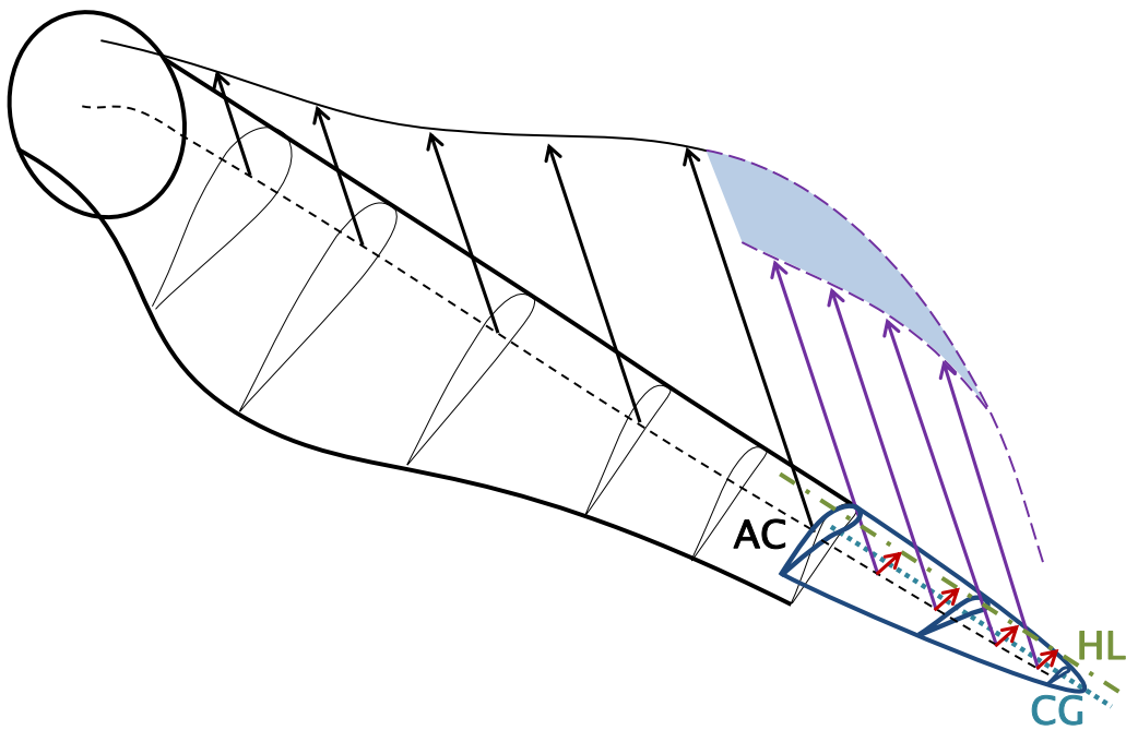
Figure 2. Wind turbine blade with articulated tip.
