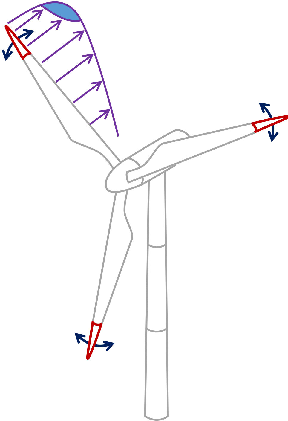
Figure 1. Articulated blade tip concept for load alleviation.
