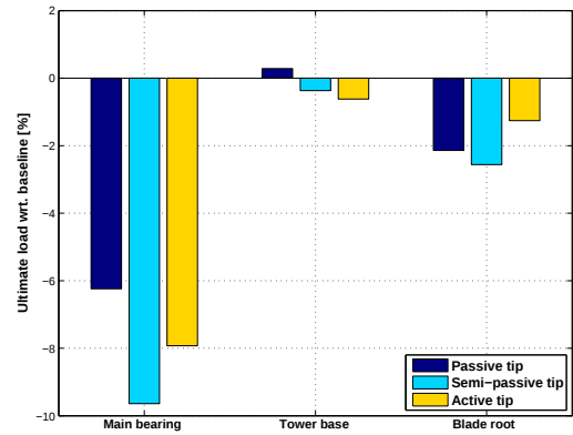
Figure 11. Percent variation of ultimate loads at verification spots with respect to baseline.
