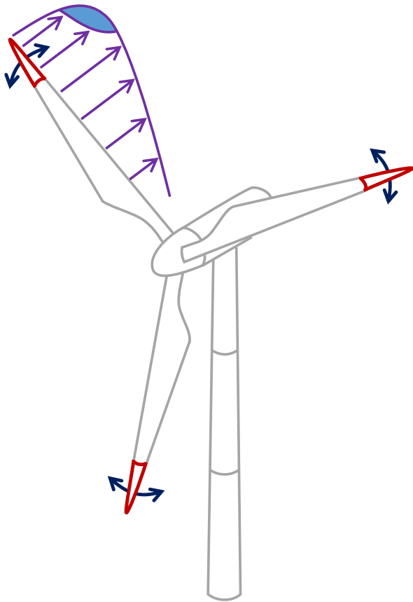
Figure 1. Articulated blade tip concept for load alleviation.
