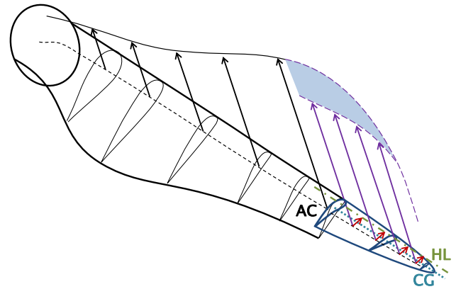
Figure 2. Wind turbine blade with articulated tip.
