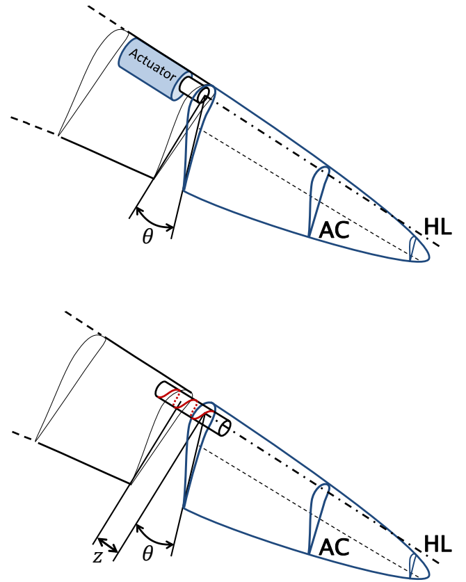
Figure 3. Top: semi-passive tip configuration. Bottom: passive tip configuration.
