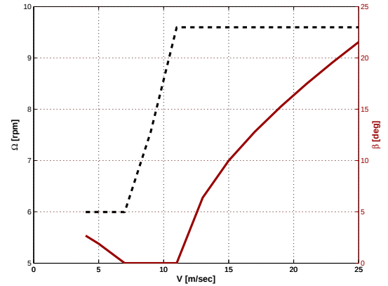
Figure 4. Rotor speed \Omega and blade pitch \beta vs. hub-height wind speed V .
