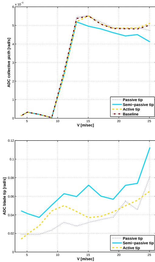
Figure 10. Top: blade pitch ADC vs. wind speed. Bottom: tip ADC vs. wind speed.
