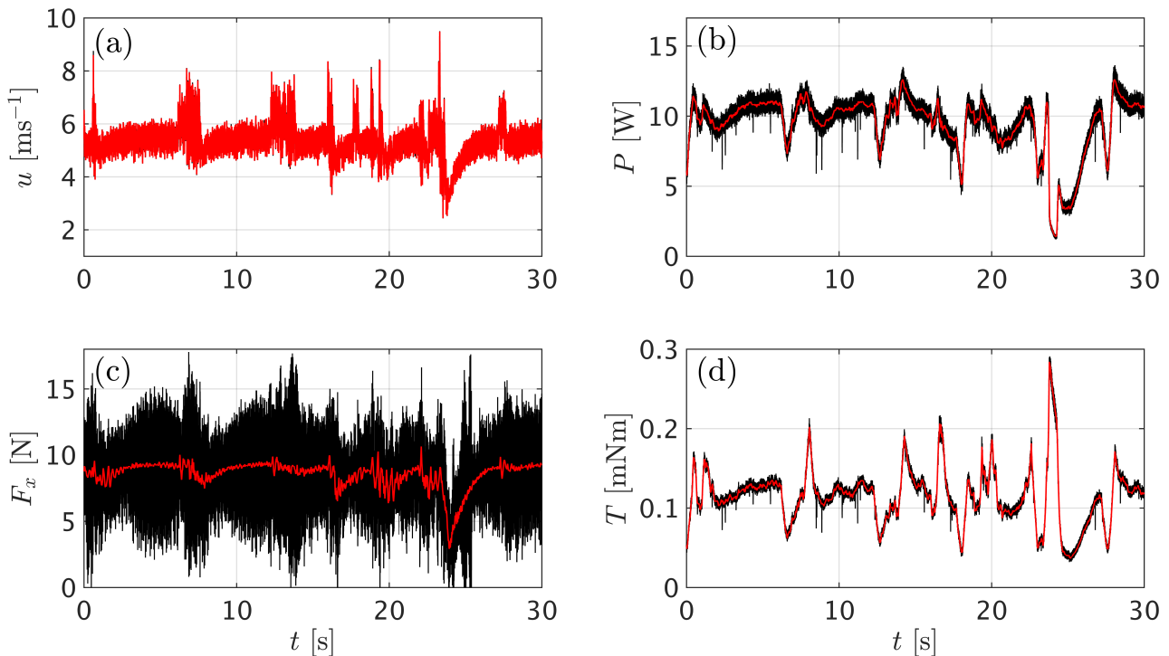
Figure 4. Original (black) and filtered (red) example time series of the wind speed (a), power (b), thrust force (c) and torque (d). The wind speed was filtered using a 6 th order Butterworth lowpass filter at 2kHz. In a similar way, the power and torque signals were filtered at 45Hz and the thrust force at 15Hz.
