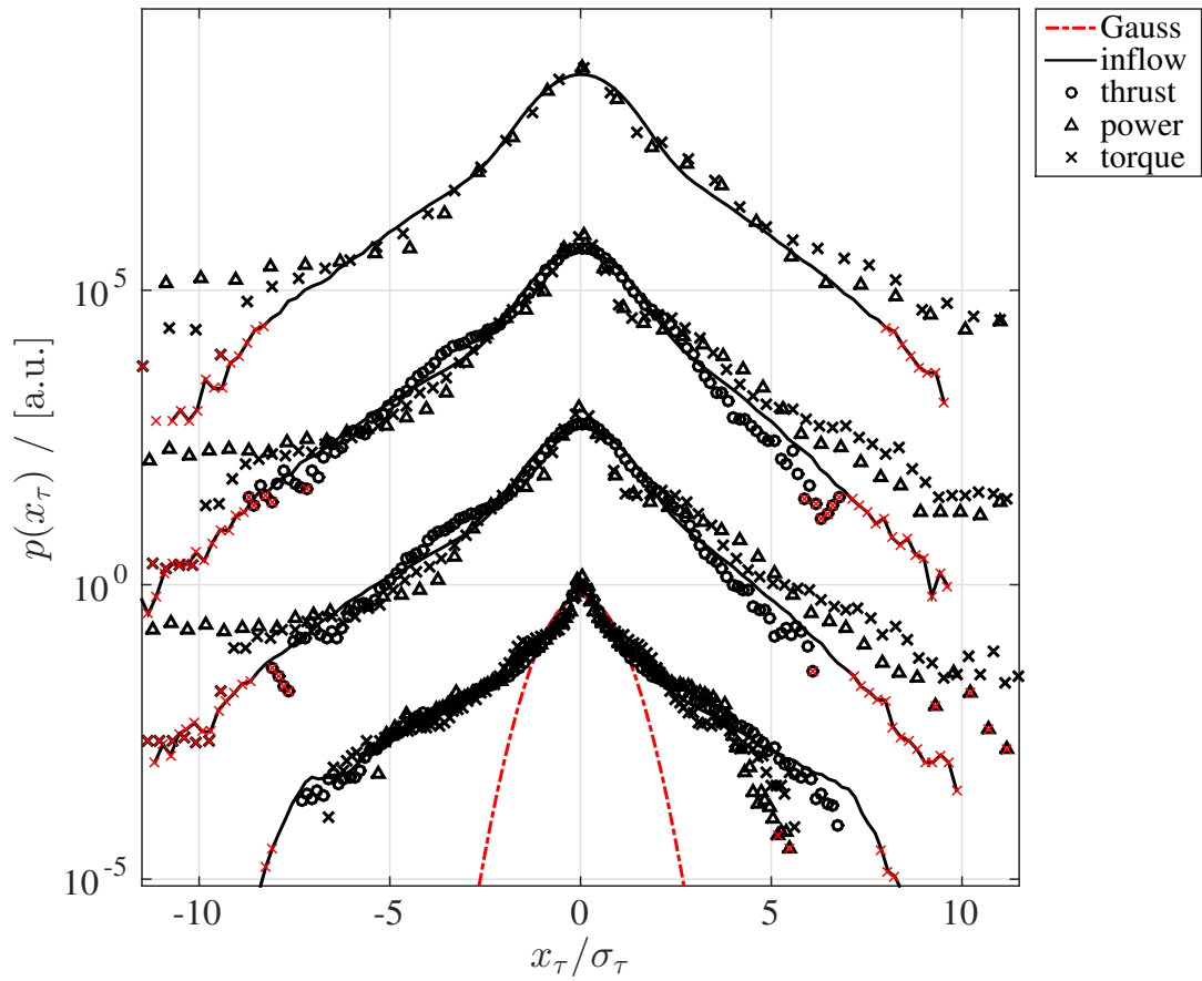
Figure 10. p(x_\tau) for the intermittent inflow condition (line, cf. Fig. 5 (A)), thrust (circles), power (triangles) and torque (crosses). Scales as in Figure 8 from top to bottom \tau = \{25 \text{ ms}, 67 \text{ ms}, 80 \text{ ms}, 2 \text{ s}\} , shifted vertically for presentation.
