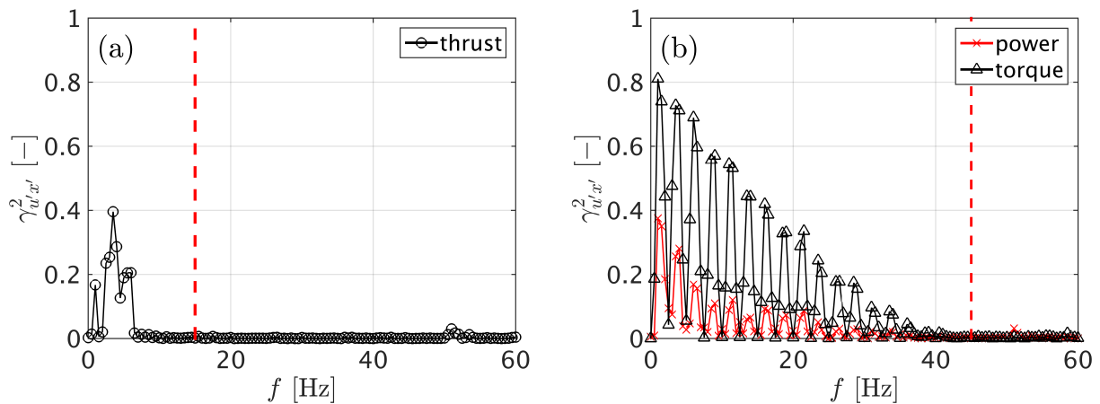
Figure 12. Magnitude-squared coherence of filtered hot wire data and thrust (a) as well as power and torque (b) respectively. 500 Hanning windows with 50% overlap were used here, as suggested by Carter et al. (1973). Graph (b) shows regular drops of \gamma^2 which are caused by a filter function within the control algorithm of the model turbine. As the controller affects the electric circuit, there is a direct connection to the electric current and therewith to the power and torque. Consequently, the effect of the filter is clearly visible in this graph.
