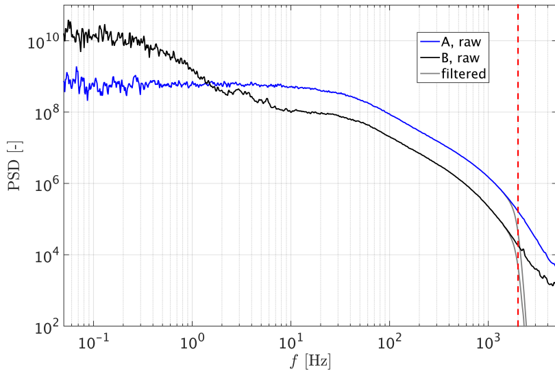
Figure 11. Power spectral density (PSD) of u(t) for the Gaussian inflow A (blue) and the intermittent inflow B (black). The effect of a 6 th order Butterworth lowpass filter at f_{cut} = 2 kHz is shown in gray. The red dashed line marks f_{cut} = 2 kHz.
