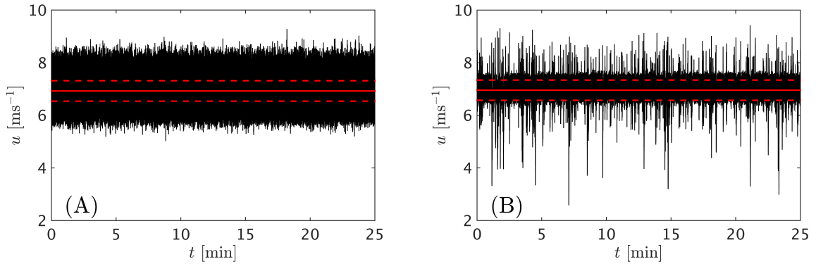
Figure 5. Velocity time series as defined in Eq. (9) of the two inflows considered, A and B. Further information is shown in Table 3. Solid red lines mark \langle u(t) \rangle and dashed red lines indicate \langle u(t) \rangle \pm \sigma_u .
