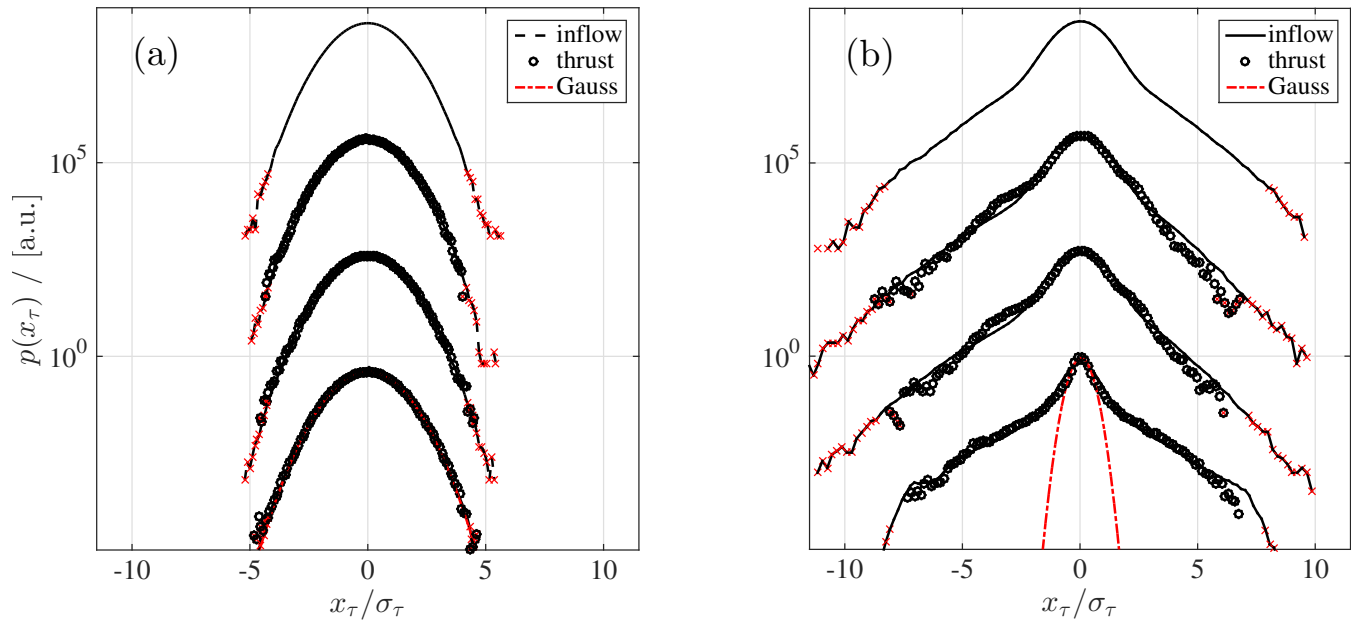
Figure 9. p(u_\tau) (lines) and p(F_\tau) (circles) for both inflow conditions Gaussian (a) and intermittent (b). Scales as in Fig. 8 from top to bottom \tau = \{25 \text{ ms}, 67 \text{ ms}, 80 \text{ ms}, 2 \text{ s}\} , shifted vertically for presentation.
