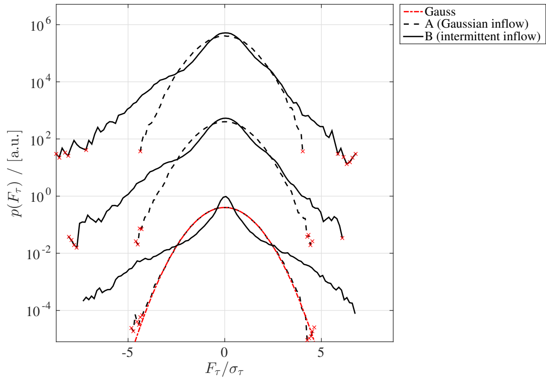
Figure 8. p(F_\tau) of the turbine's thrust force (in main flow direction) exposed to the inflow conditions A (dashed) and B (solid), for \tau = \{67 \text{ ms}, 80 \text{ ms}, 2 \text{ s}\} from top to bottom. The different scales are shifted vertically for presentation.
