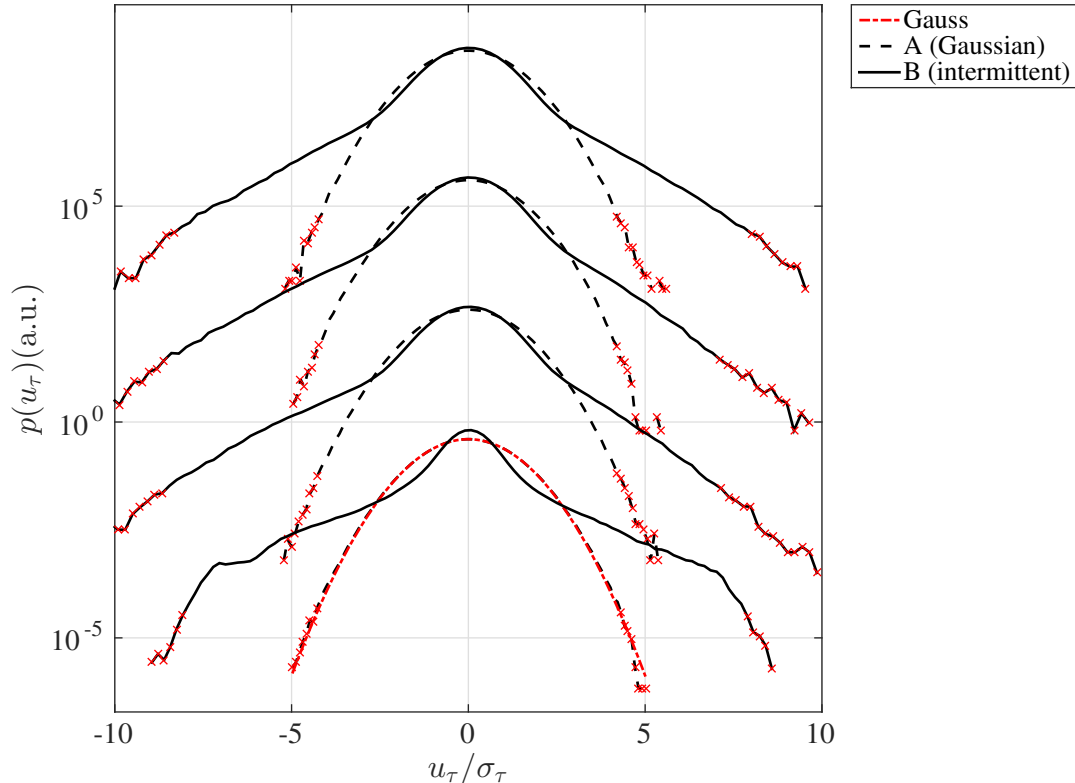
Figure 7. p(u_\tau) of both velocity time series shown in Fig. 5, A (dashed) and B (solid), for \tau = \{25 \text{ ms}, 67 \text{ ms}, 80 \text{ ms}, 2 \text{ s}\} from top to bottom. The different scales are shifted vertically for presentation. A Gaussian fit (dashed red line) of p(u_{\tau=2\text{s}}) for inflow A is added to guide the eye.
