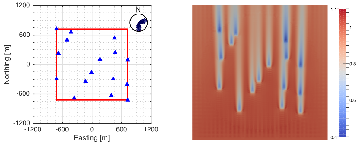
Figure 7. Optimal layout (left) and flow field (right) for the boomerang test case with the wind rose binned into 36 inflow directions and a uniform hub-height velocity of 8 m/s. The wind rose is shown in the upper right corner of the left panel, and the site boundary is shown by a solid red line. Turbine locations are denoted by blue triangles. The flow field in the right panel is normalized by the incoming hub-height velocity of 8 m/s and shows results for an inflow wind from the south.
