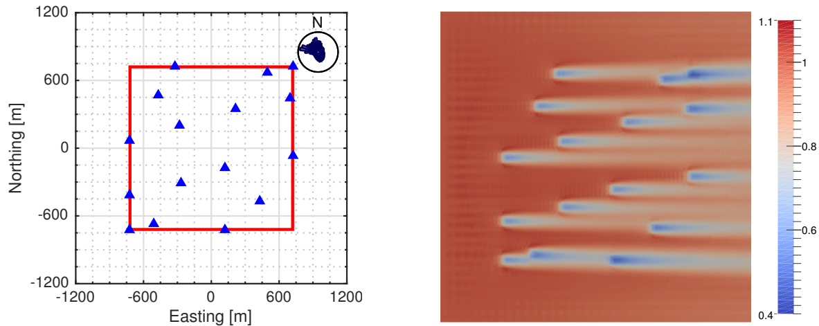
Figure 8. Optimal layout (left) and flow field (right) for the NWTC M2 8 m/s test case with the wind rose binned into 36 inflow directions. The wind rose is shown in the upper right corner of the left panel, and the site boundary is shown by a solid red line. Turbine locations are denoted by blue triangles. The flow field in the right panel is normalized by the incoming hub-height velocity of 8 m/s and shows results for an inflow wind from the west.
