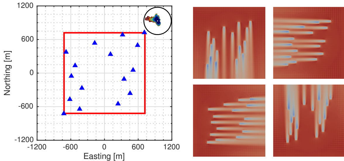
Figure 9. Optimal layout (top left) and flow fields resulting from a full AEP optimization using data from the M2 mast at NWTC. Differences in both wind speed and wind direction are accounted for in the optimization, and the wind rose used is shown in the top right corner of the layout plot. In the top left panel, the site boundary is shown by a solid red line and turbine locations are denoted by blue triangles. Flow fields are shown for inflow winds from the west (top right), south (bottom right), and north (bottom left).
