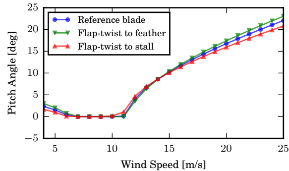
Figure 4. Pitch angles over wind speed for the reference and flap-twist to feather and stall coupled blades with coupling coefficients \gamma_y = \pm 0.1 constant along the blade.
