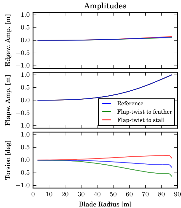
Figure 6. Structural mode shape of the first flapwise mode for the reference blade, and flap-twist coupled blades with constant coupling coefficients of \gamma_y = \pm 0.1 . Positive coupling coefficients denote twist to stall for flapwise deflection towards the suction side. The amplitudes are normalised to 1 m tip deflection in the flapwise direction.
