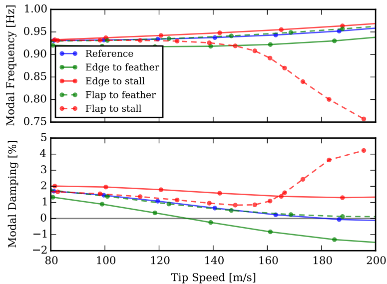
Figure 15. Campbell diagram of modal frequency (top) and damping (bottom) for the first edgewise mode in a runaway scenario. Coupling coefficients are \gamma_{x/y} = \pm 0.1 constant along the blade.
