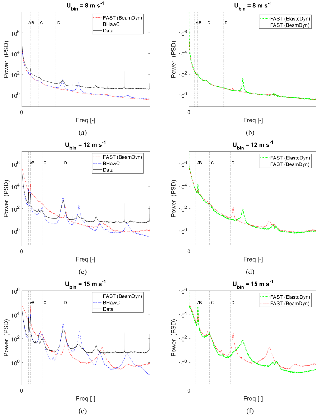
Figure 12. PSDs of the electrical power. The three sets of graphs represent the ensemble-averaged PSDs from the inflow velocity bins at 8 \text{ m s}^{-1} (top), 12 \text{ m s}^{-1} (center), and 15 \text{ m s}^{-1} (bottom).
