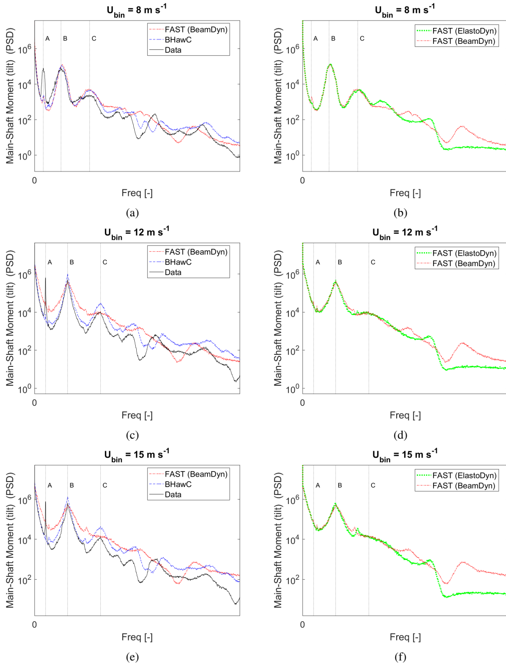
Figure 20. PSDs of the main-shaft bending moment—tilt (nonrotating coordinate system). The three sets of graphs represent the ensemble-averaged PSDs from the inflow velocity bins at 8 \text{ m s}^{-1} (top), 12 \text{ m s}^{-1} (center), and 15 \text{ m s}^{-1} (bottom).
