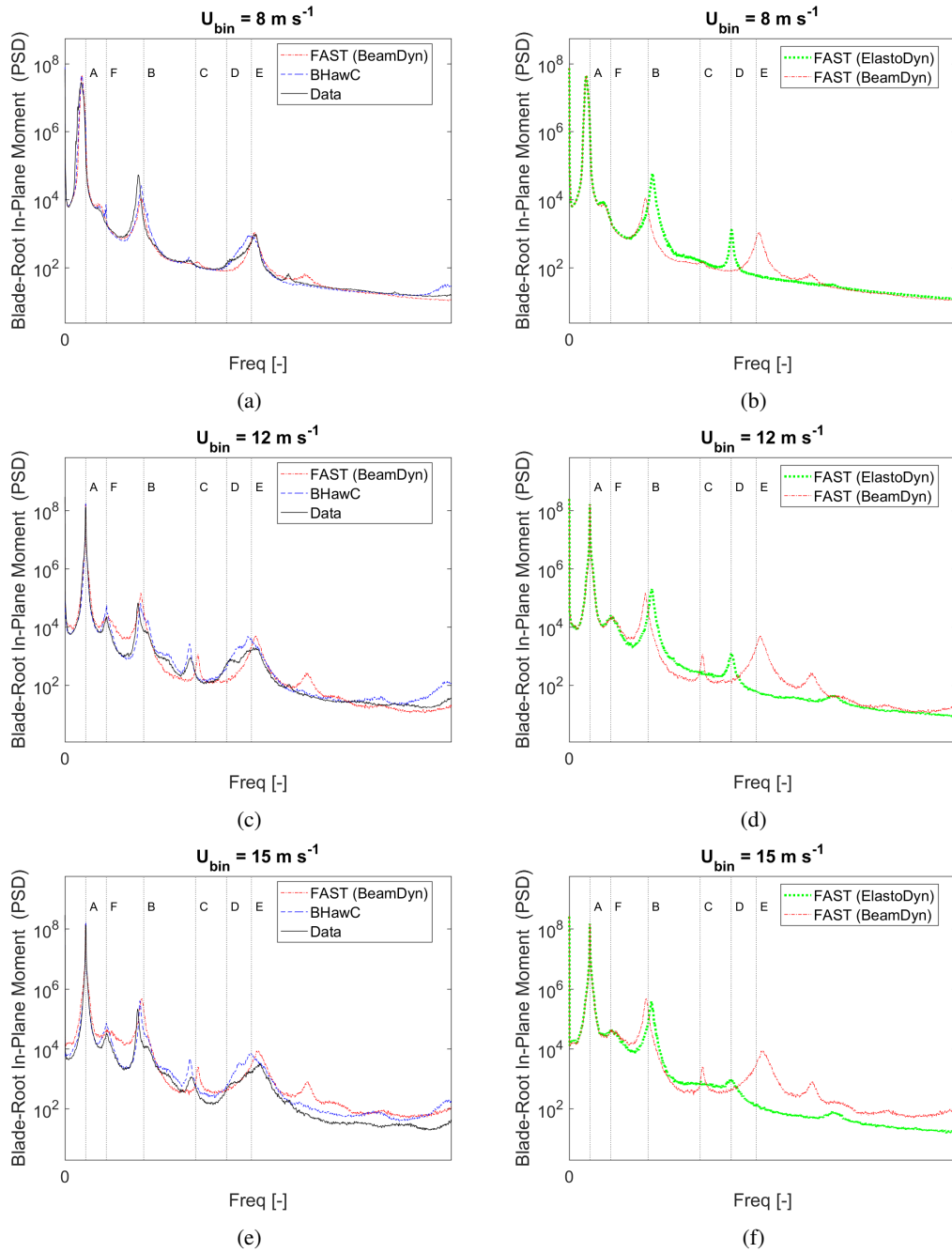
Figure 17. PSDs of the blade-root in-plane bending moments. The three sets of graphs represent the ensemble-averaged PSDs from the inflow velocity bins at 8 \text{ m s}^{-1} (top), 12 \text{ m s}^{-1} (center), and 15 \text{ m s}^{-1} (bottom).
