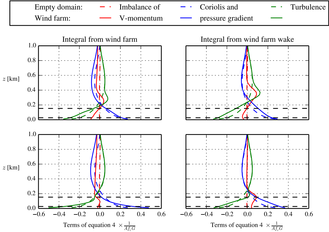
Figure 7. V -Momentum balance. Top: wind farm represented by 25 ADs, where rotor area is shown as black dashed lines. Bottom: wind farm represented by a high roughness. Left: integral taken from wind farm area. Right: integral taken from near wind farm wake. Dashed lines represent the results from an empty domain.
