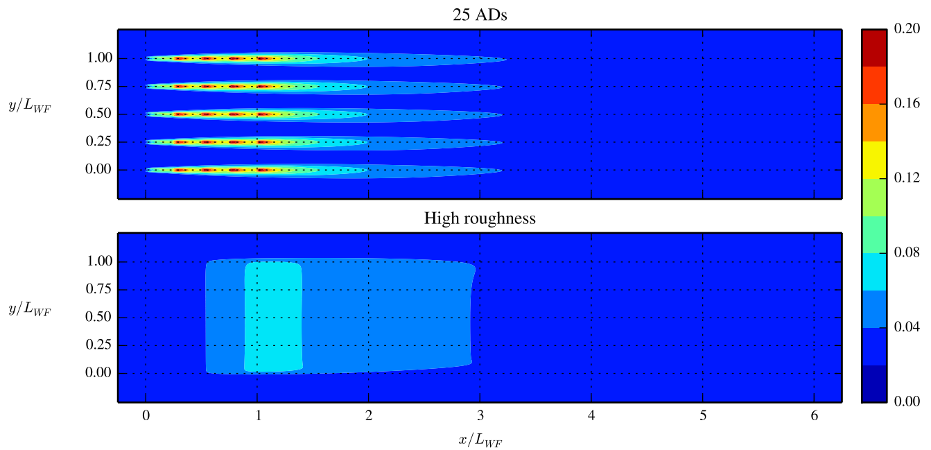
Figure 5. Turbulence intensity at hub height. Top: Wind farm modeled with 25 ADs. Bottom: Wind farm modeled as a high roughness.
