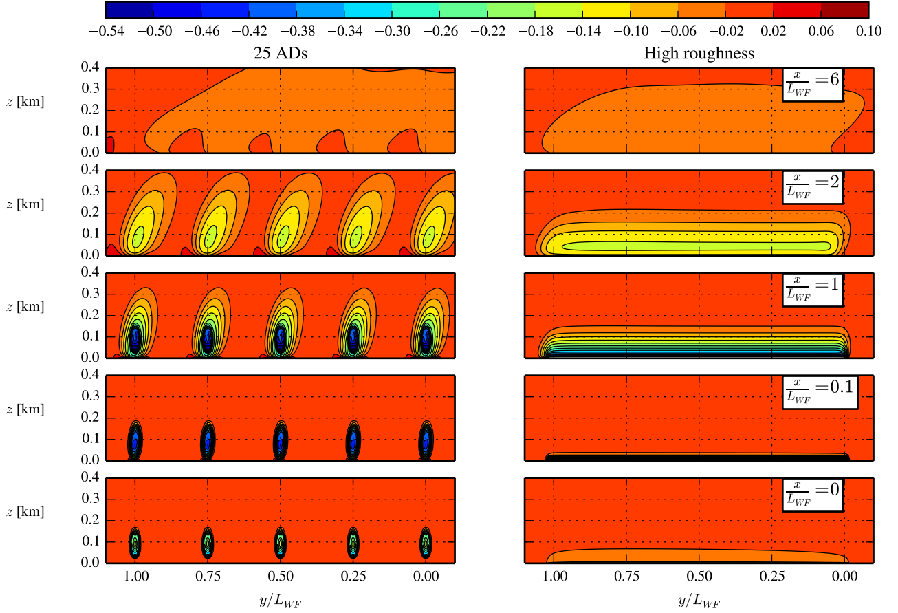
Figure 6. Stream-wise velocity subtracted and normalized by the free-stream (U - U_{\text{inflow}})/U_{\text{inflow}} at several downstream cross planes. Left: wind farm is represented by 25 ADs. Right: wind farm is represented by a high roughness. Wind farm ends at x/L_{WF} = 1 .
