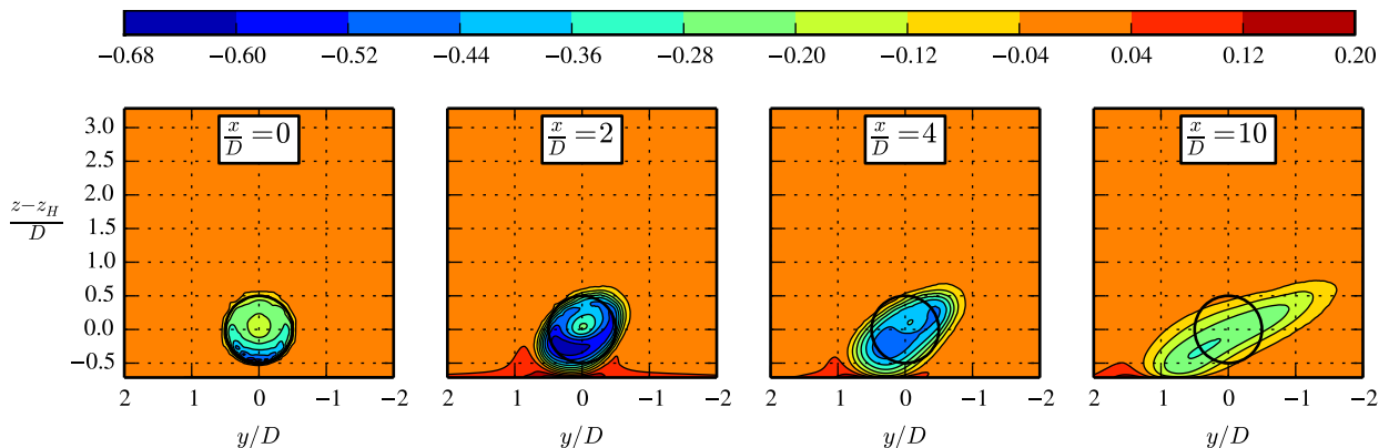
Figure 10. Stream-wise velocity subtracted and normalized by the free-stream (U - U_{\text{inflow}})/U_{\text{inflow}} at several downstream cross planes for a single wake in a shallow ABL. AD is shown as a black circle.
