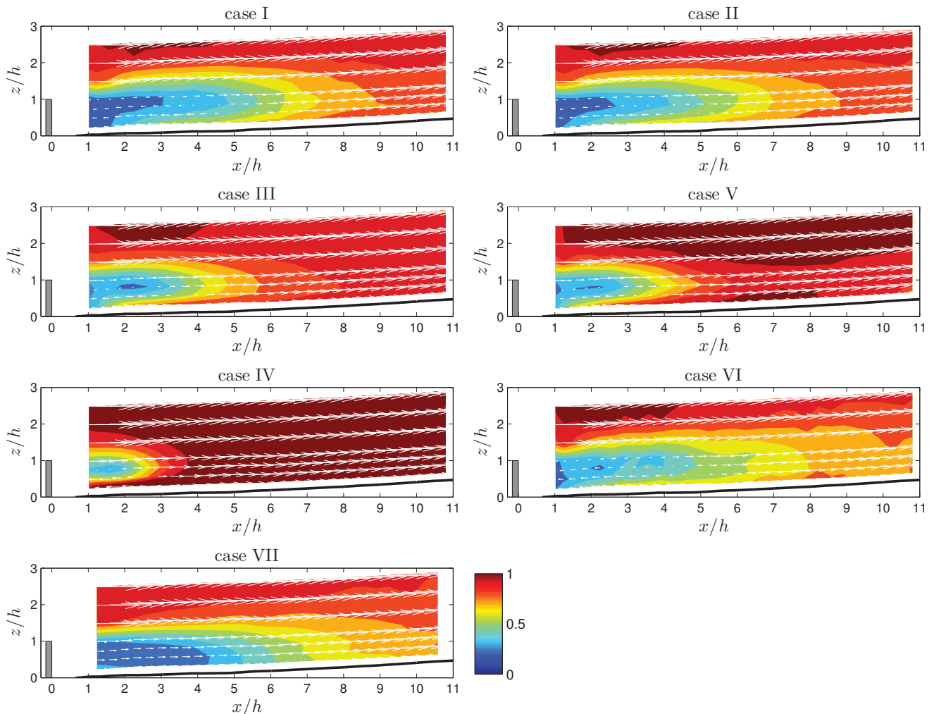
Figure 8. Averaged wind-speed ratio \langle \tilde{U}(x, z)_{ws} \rangle / \langle U_o(z) \rangle (colorbar) behind the fence for a number of cases. Vectors indicate the magnitude and sign of the ensemble-averaged u -component
