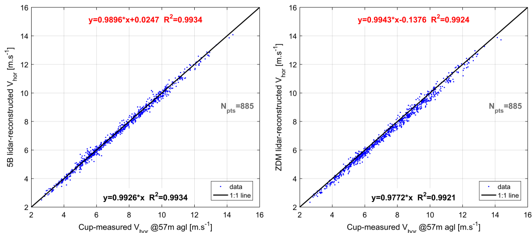
Figure 10. Comparison between mast-measured and lidar-estimated horizontal wind speed at 57.5 m height agl and 2.5D_{rot} using short-range measurements. Left: 5B-Demo lidar, using 5 LOS and 4 ranges. Right: ZDM lidar, using 6 LOS and 3 ranges.
