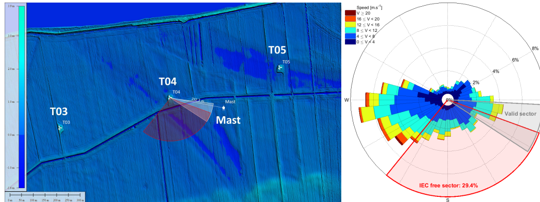
Figure 3. Left: elevation map in the vicinity of T04, Nørrekær Enge wind farm. Map: DHM/Terrain (0.4 m grid). Source: Styrelsen for Dataforsyning og Effektivisering . Right: wind rose during the NKE campaign, measured by the top-mounted cup anemometer and wind vane.
