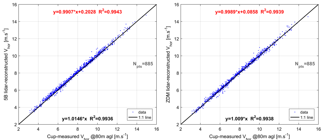
Figure 7. Comparison between mast-measured and lidar-estimated horizontal wind speed at 80 m height agl.
