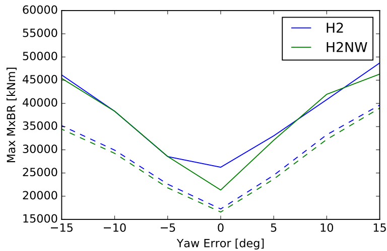
Figure 13. Maximum flapwise blade root bending moment for wind directions between -15 and 15 degrees. Dashed lines show the mean of the maximum values for the 36 different seeds, the solid lines the maximum of the maxima.
