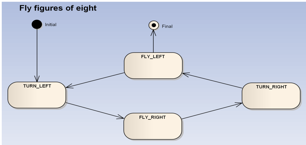
Figure 4. Finite sub-state diagram showing the sub-state and the transitional condition of the figure eight controller. This sub-state machine is active in the state FIG-8 of the high-level controller. The states LAST-LEFT and LAST-RIGHT are omitted for simplicity Fechner (2016).
