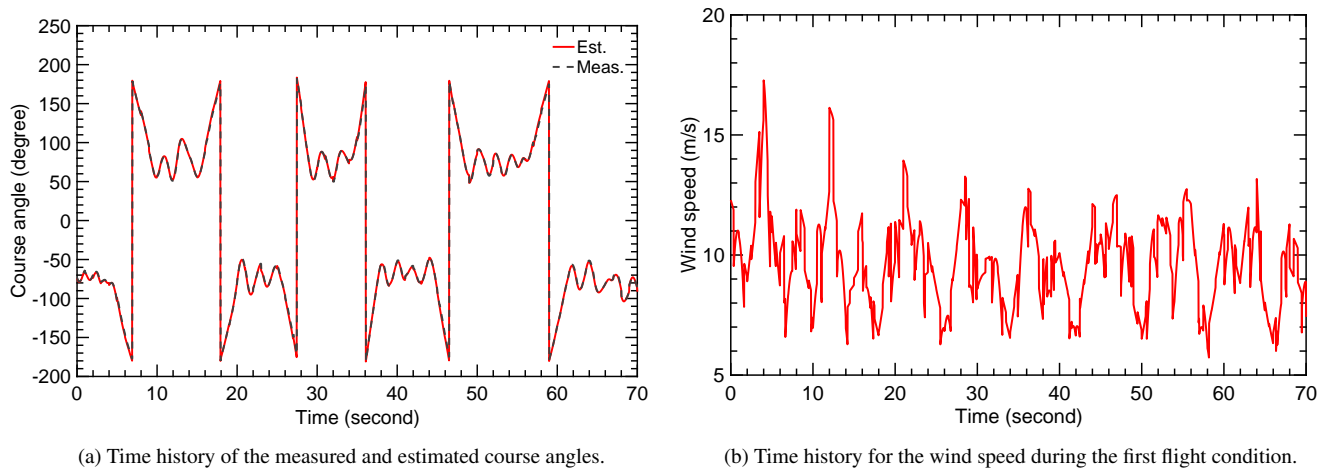
Figure 11. Time history for the wind speed and course angles.
