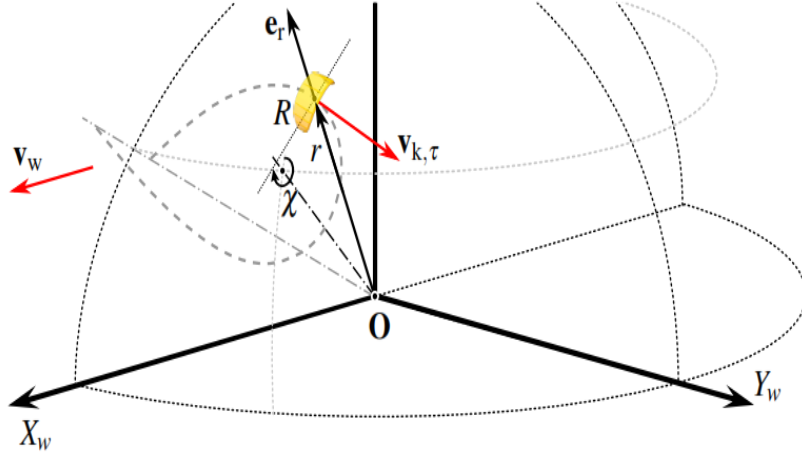
Figure 5. Schematic to show the turn rate law of the kite as a function of the angular velocity and turn radius Fechner (2016).
