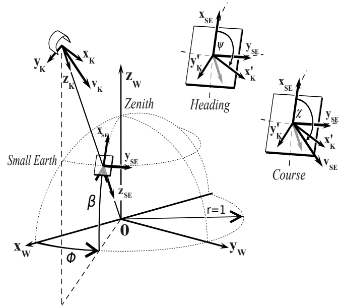
Figure 2. Small Earth Reference Frame. The position of the kite is projected onto a half sphere with a radius of one. The elevation angle \beta and the azimuth angle \phi describe the position of the kite, the angle \psi , and its orientation. The course angle \chi is the angle between the direction toward the zenith and the velocity vector of the center of mass of the kite as projected on the tangential plane touching the position of the kite on the half sphere Fechner (2016).
