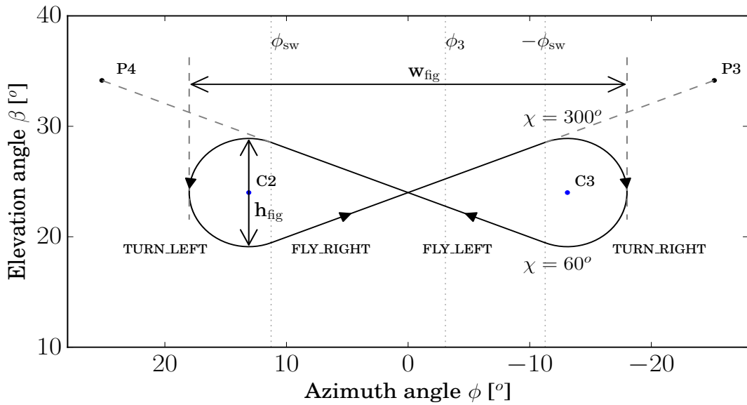
Figure 3. Four-step flight path planner for flying a figure eight: First turn left, then steer toward P_3 , then turn right and finally steer toward P_4 Fechner (2016).
