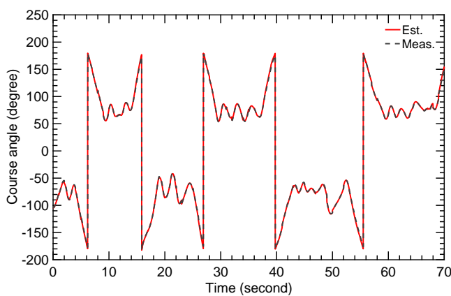
(a) Time history of the measured and estimated course angles.
