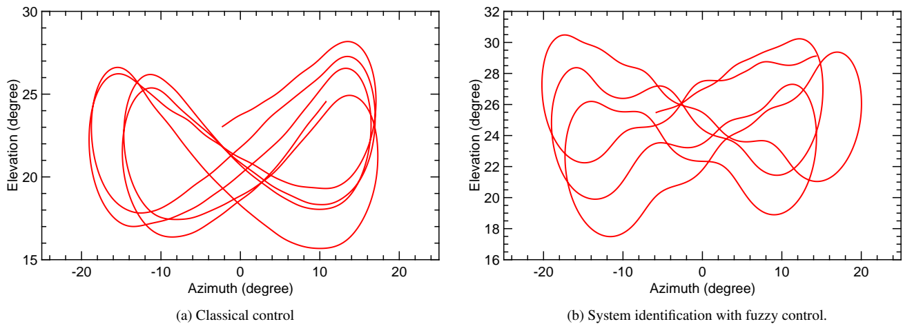
Figure 10. Simulation results for the azimuth and elevation angles during 70 seconds.
