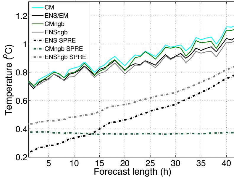
Figure 5. Unbiased forecast error std for all uncertainty quantification approaches for the temperature in ^{\circ}\text{C} and the spread, SPRE , for the three approaches consisting of multiple forecasts as a function of increasing forecast length. The std is calculated for the average forecast in case of multiple forecasts i.e. approach CMngb, ENS and ENSngb.
