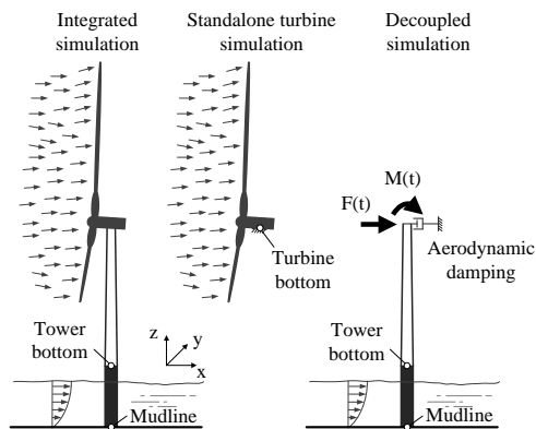
Figure 1: Offshore wind turbine and simulation methods
