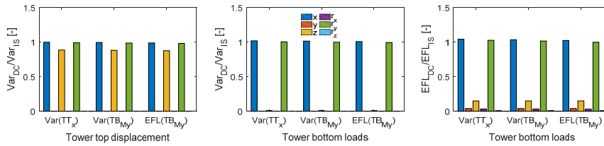
Figure 6: Response for tower top displacements and tower bottom loads for wind speed of 8m/s and DC II.
