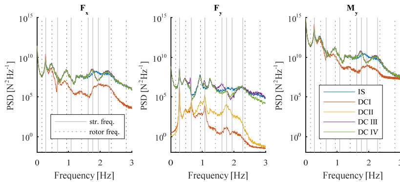
Figure 17: PSD for forces and moment at tower bottom for wind speed of 8 m/s
