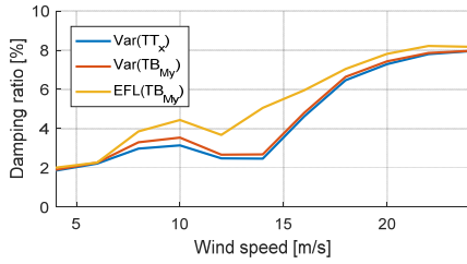
Figure 5: Damping ratios optimized for different output for DC II.
