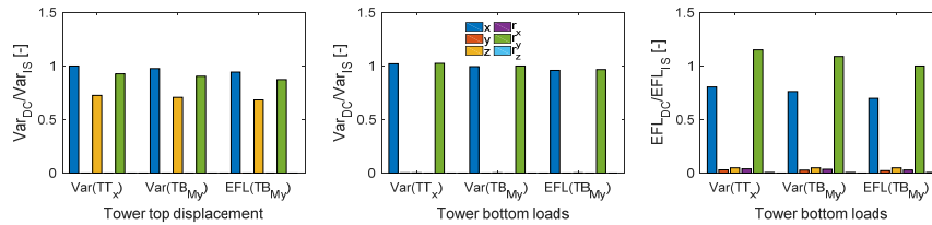
Figure 3: Response for tower top displacements and tower bottom loads for DC I and a wind speed of 8 m/s. Damping coefficients matching the variance of the tower top displacement in x-direction ( Var(TT_x) ), the variance of the tower bottom bending moment around the y-axis ( Var(TB_{My}) ), and the EFL of the tower bottom bending moment around the y-axis ( EFL(TB_{My}) ) are chosen for the decoupled analysis. Each bar stands for a displacement or force/moment in one out of the six degrees of freedom.
