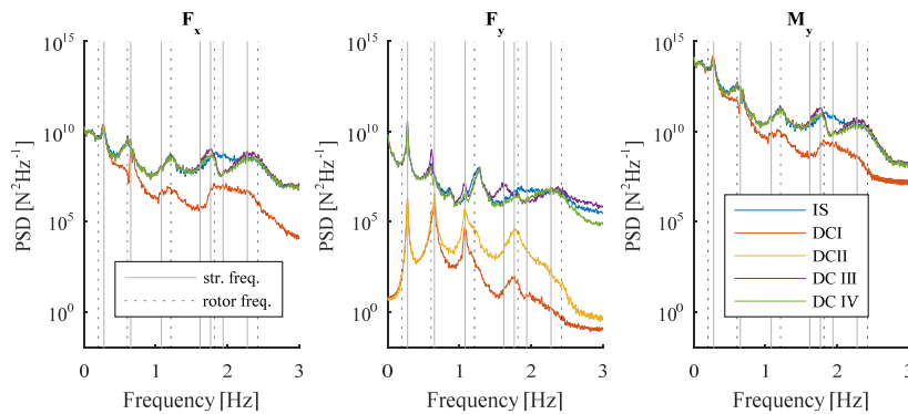
Figure 18: PSD for forces and moment at tower bottom for wind speed of 20 m/s.
