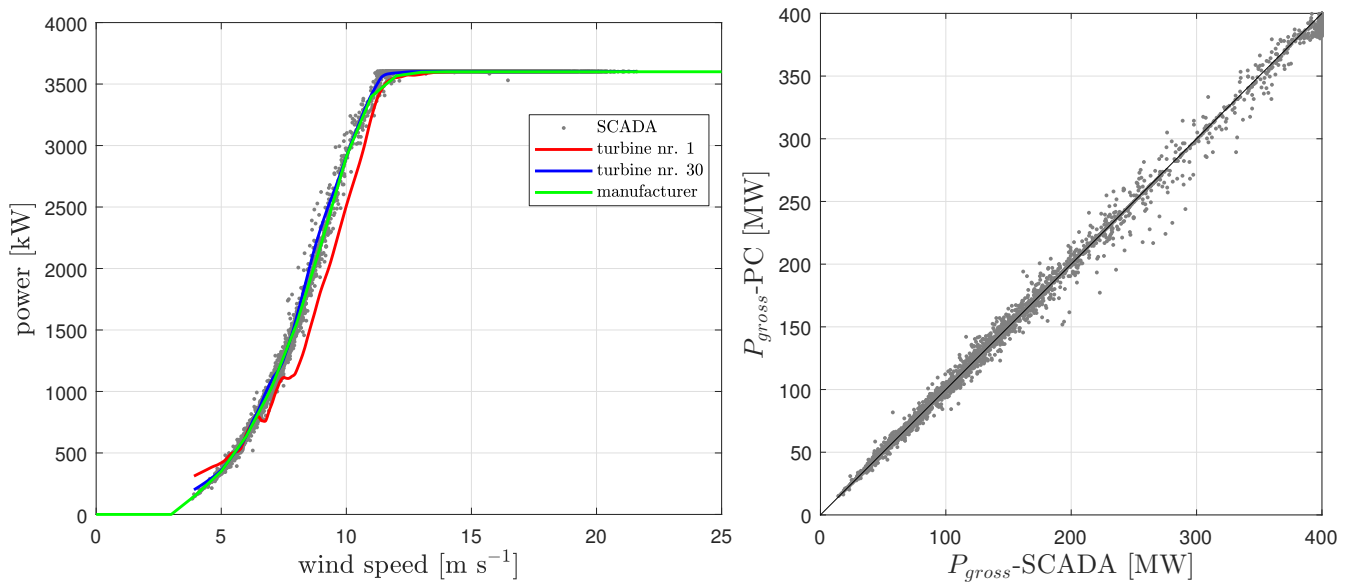
Figure 8. (Left) power curve of the turbines at the Anholt wind farm derived from the SCADA of free-stream turbines compared to the manufacturer power curve. (Right) gross wind-farm power derived from the SCADA for the free-stream turbines compared to that derived from the power curve (PC)
