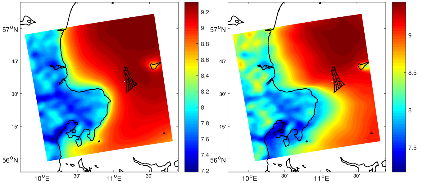
Figure 4. WRF-simulated mean wind speed at hub height on the Kattegat area where the Anholt wind farm is deployed for the year 2014. All data are shown in the left frame and data within the directions 270 \pm 30^\circ at the position of turbine nr. 15 in the right frame. Colorbars are in \text{m s}^{-1}
