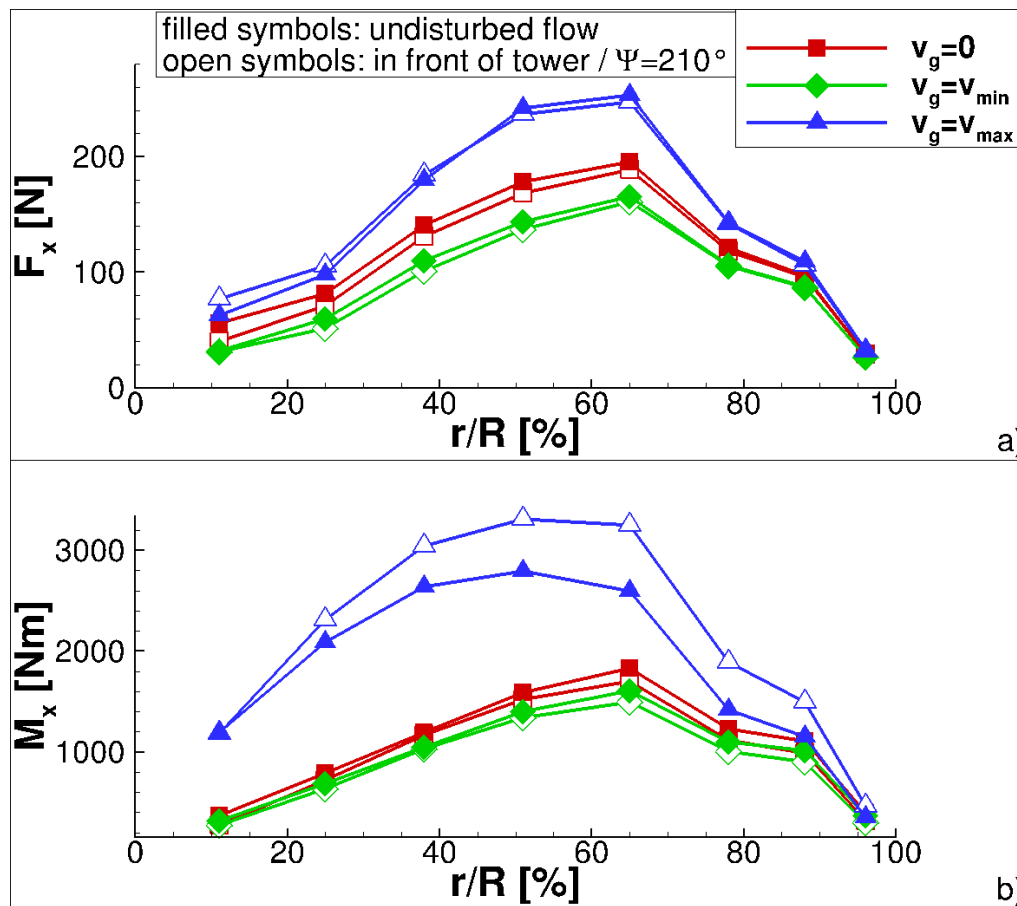
Fig. 3. radial distribution of rotor thrust and torque
