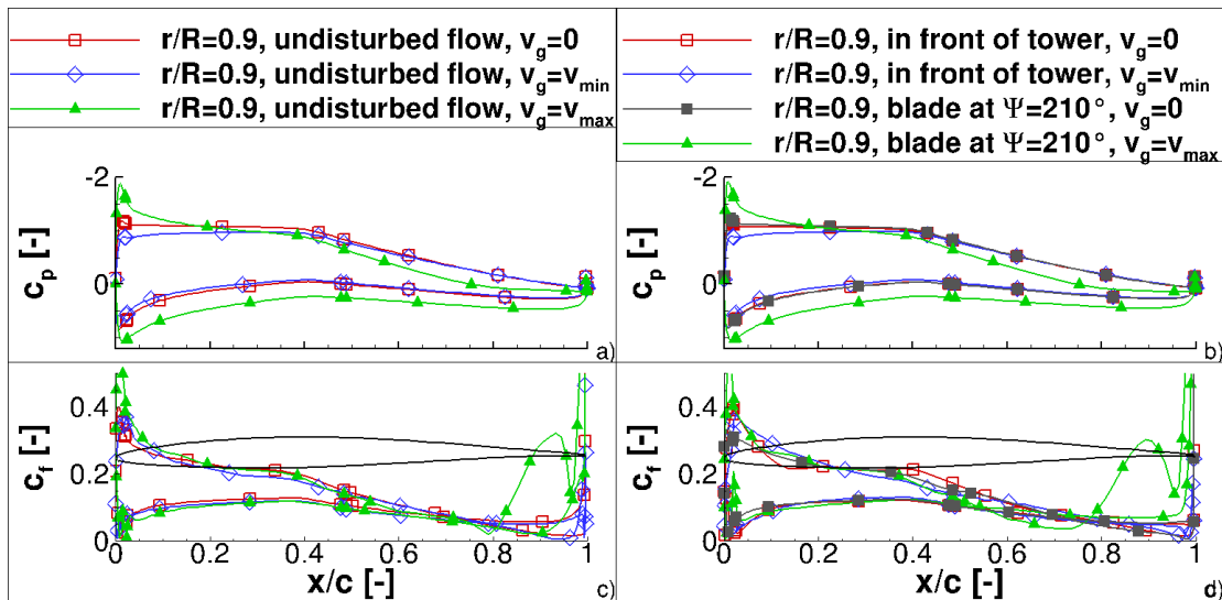
Fig. 2. pressure coefficient and friction force coefficient
