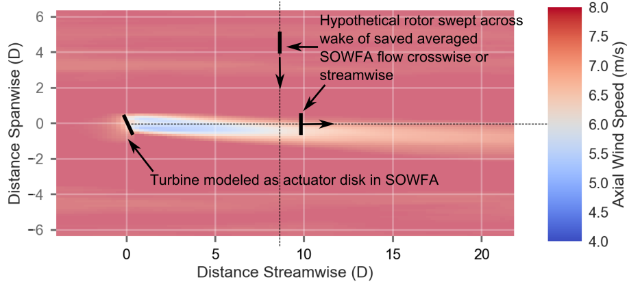
Figure 1. Diagram of the method used in the paper. In this example, showing the flow as viewed from above, a single turbine is included in a SOWFA simulation. A period of 1600 seconds of the flow is averaged and then the hypothetical turbine rotor is scanned across this averaged flow to compute the power that would have been produced by a turbine at a given location.
