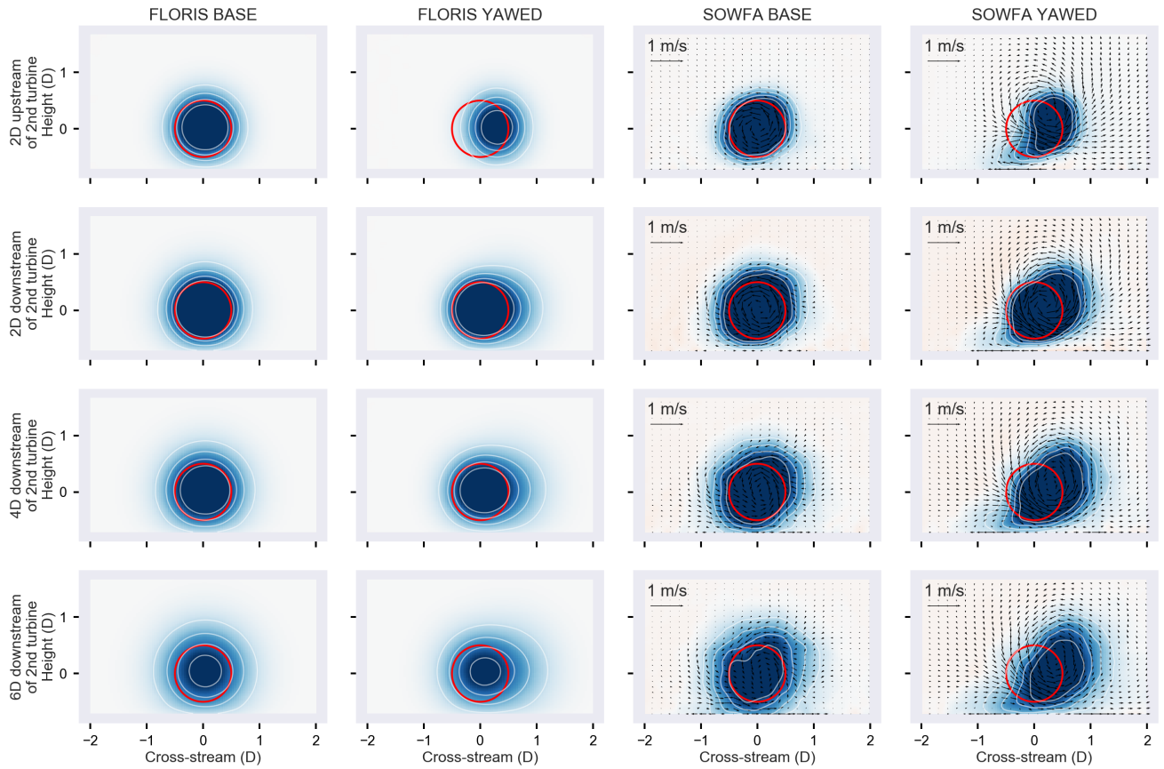
Figure 7. Cut-through visualizations of FLORIS and SOWFA 2D in front of second turbine (top row) and behind the second turbine (remaining rows).
