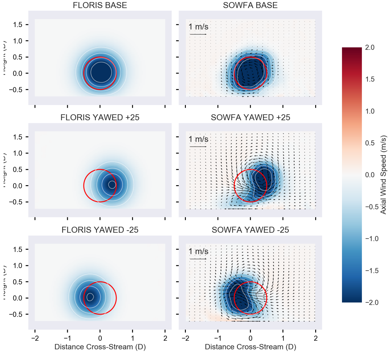
Figure 3. Cut-through of SOWFA flow (viewed from upstream), minus the background flow, at a distance of 7 diameters behind the turbine for baseline and yawed 25° and -25°. Deficit in axial flow is shown in blue, saturating at a deficit of 2 m/s to broadly show the wake area. For the SOWFA cases, the in-plane flow is visualized by arrows whose relative size indicates the strength of the flow. Red circles indicate a rotor located directly downstream of the turbine.
