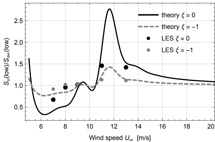
Figure 7. Change of low frequency ( f < 0.03 Hz) spectral power of the longitudinal velocity component in the rotor plane and one radius upstream. The dots are the LES simulations while the lines are the quasi-steady model based on Eqs. (2) and (3)
