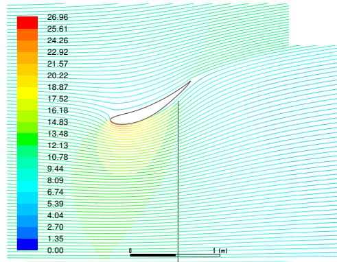
Figure 11. Flow field of a near-optimal design based on C_{P,tot}
