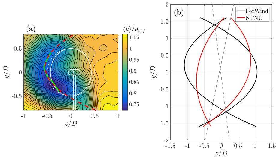
Figure 12. (a): Example of parameterizing the curled shape of the velocity deficit. The green markings show minimal velocities of a polynomial function used to fit the interpolated data points in a horizontal line, y = \text{const.} The red, dashed line shows a quadratic fit based on the green markings. (b): Visualization of the curled shapes of the velocity deficits. For both turbines, the cases \gamma = \pm 30^\circ are shown. Dashed lines show a visualization of the wakes tilt, connecting the respective intersections of the curves.
