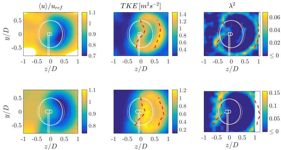
Figure 13. \langle u \rangle / u_{ref} (left column), TKE (center column) and \lambda^2 (right column) for \gamma = -30^\circ behind the NTNU turbine (top row) and the ForWind turbine (bottom row). The time scale for \lambda^2 corresponds to the length scale of the rotor diameter. The red marks show the approximation of the respective parameter's radial extension based on \mu \pm 1\sigma_u and \mu \pm 2\sigma_u as described in Section 3.1.
