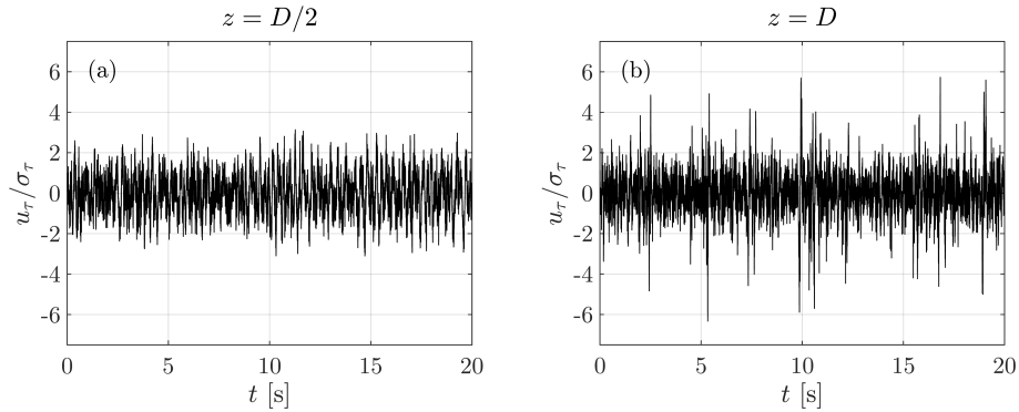
Figure 9. u_\tau(t) at z = D/2 (a) and z = D (b) behind the ForWind turbine, cf. Figures 7(b) and 8(b). \sigma_\tau is the standard deviation of u_\tau .
