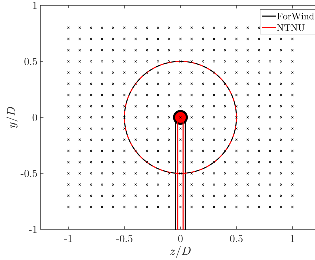
Figure 3. Non-dimensional measurement grid behind the rotor for \gamma = 0^\circ . The respective contours of the turbines are shown in black (ForWind) and red (NTNU).
