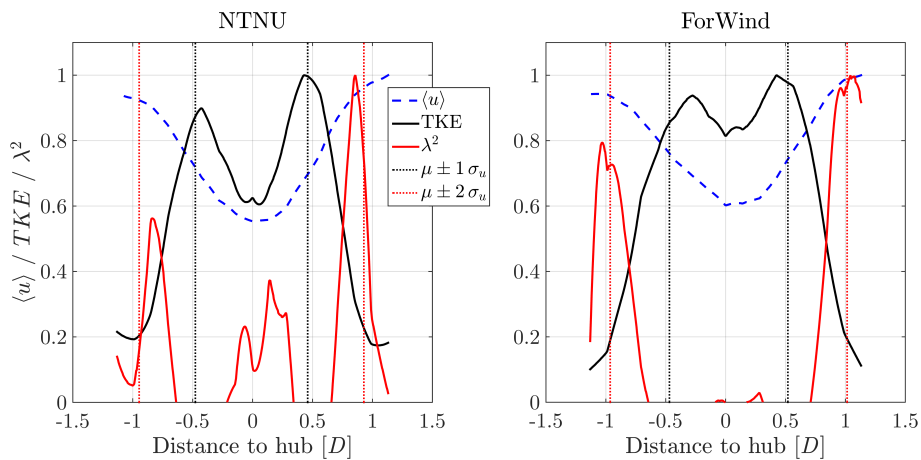
Figure 10. Diagonal cuts on the line y = z through the contour plots for \gamma = 0^\circ . Values are normalized to their respective maximum. The vertical dotted lines mark \mu \pm 1\sigma_u (black) and \mu \pm 2\sigma_u (red) of a Gaussian fit through the velocity deficit shown in blue.
