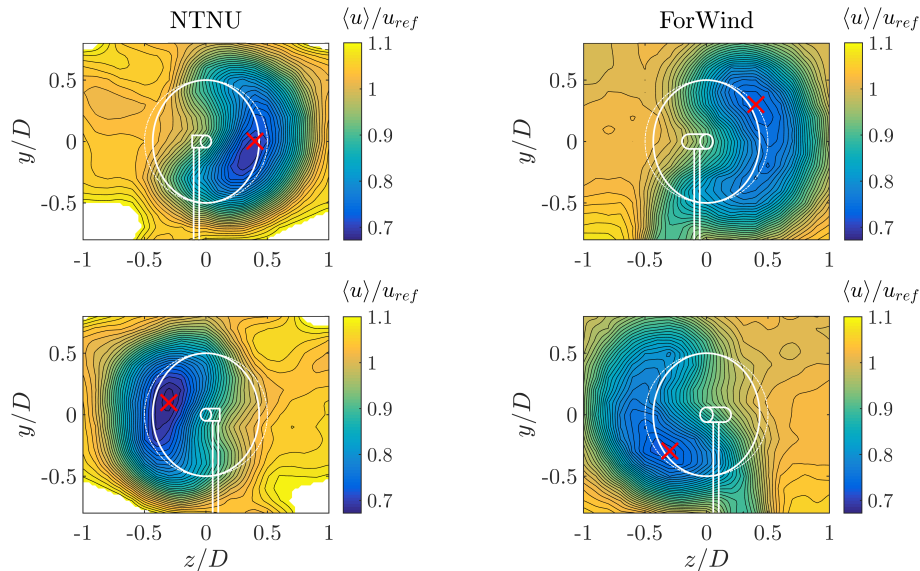
Figure 11. \langle u \rangle / u_{ref} during yaw misalignment. Top row: \gamma = -30^\circ , bottom row: \gamma = 30^\circ . Left column: NTNU turbine, right column: ForWind turbine. The solid white lines indicate the contours of the respective turbine, while the dashed lines denote the rotor area without yaw misalignment. The red \times marks the position of minimum measured velocity \langle u \rangle . Values exceeding 1.1 are masked for better comparison.
