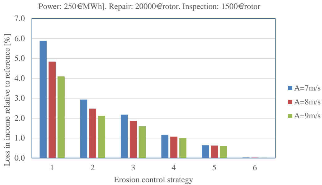
Figure 21: Loss of income due to erosion, inspection and repair. Energy: 250€MWh]. Repair: 20000€rotor. Inspection: 1500€rotor.
