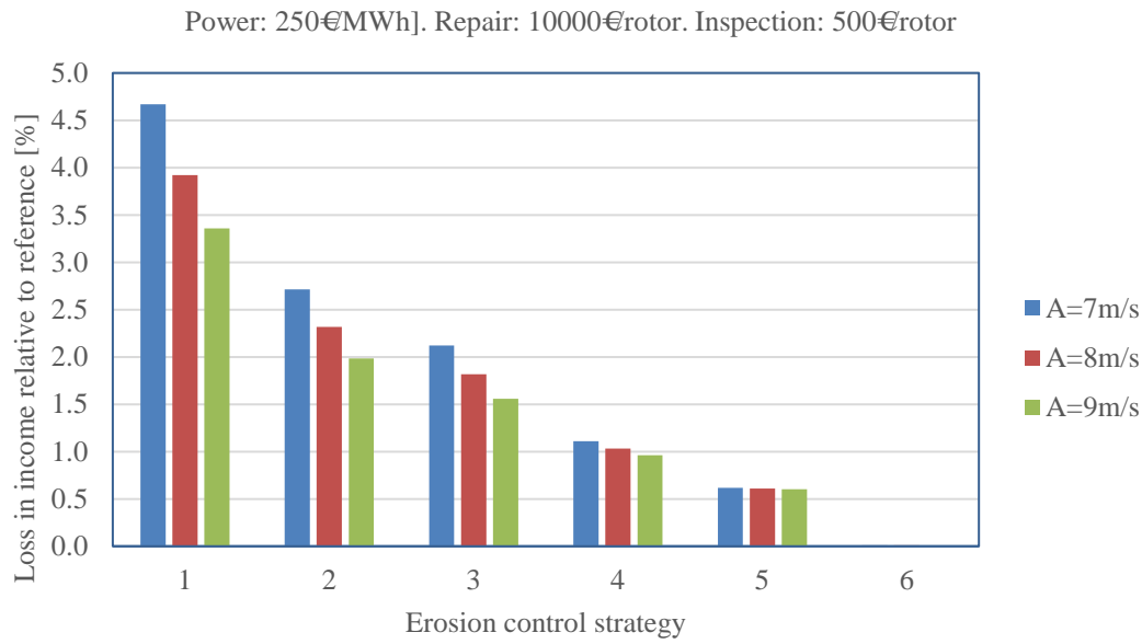
Figure 20: Loss of income due to erosion, inspection and repair. Energy: 250€MWh]. Repair: 10000€rotor. Inspection: 500€rotor.
