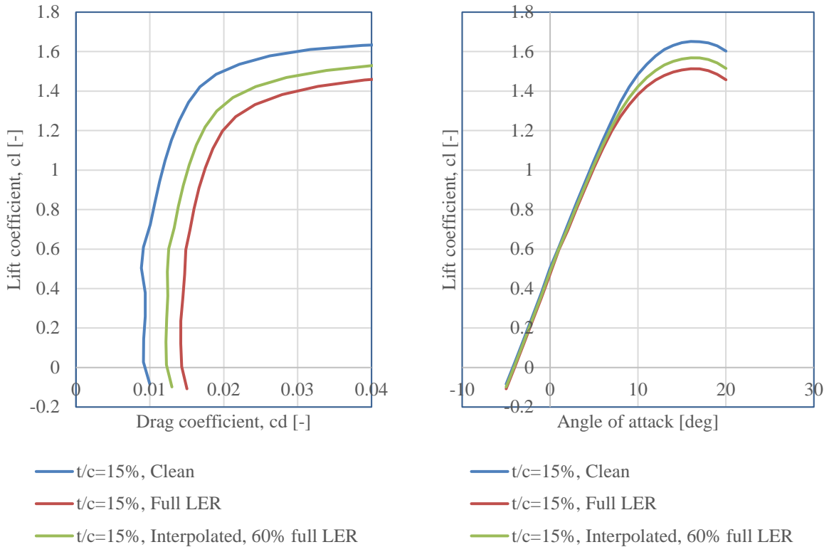
Figure 13: Airfoil characteristics of the outer part of the blade: blue = clean blade , red = full leading edge roughness and green = 60% of full leading edge roughness. Left: Lift coefficient, c_l , as a function of drag coefficient, c_d . Right: Lift coefficient, c_l , as a function of angle-of-attack, AOA.
