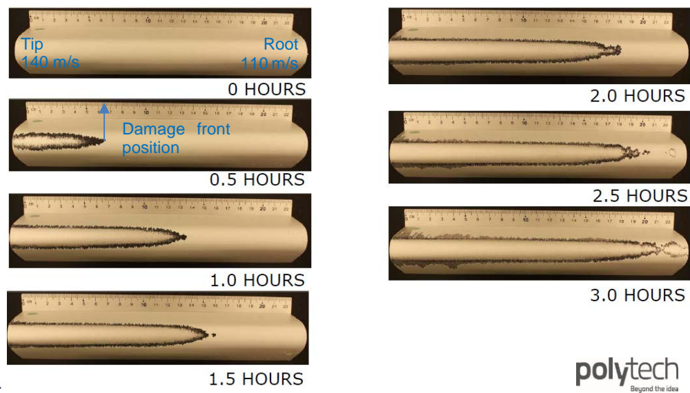
15 Figure 2: Whirling arm rain erosion test specimen photographed at 30 minutes intervals during 3 hours of testing.
