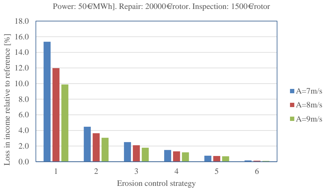
Figure 19: Loss of income due to erosion, inspection and repair. Energy: 50€/MWh]. Repair: 20000€/rotor. Inspection: 1500€/rotor
