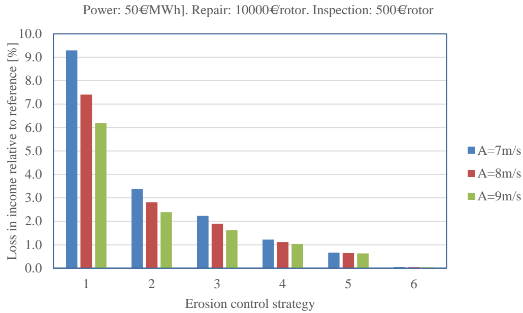
Figure 18: Loss of income due to erosion, inspection and repair. Energy: 50€/MWh]. Repair: 10000€/rotor. Inspection: 500€/rotor.
