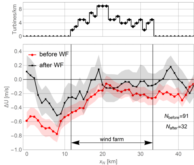
Figure 11: Wind speed difference similar to Figure 9 for short fetch situations with wind directions between 255° and 285°.
