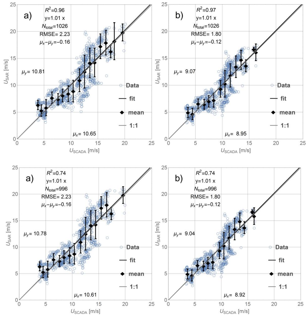
Figure 4: Comparison between SCADA derived wind speeds ( U_{SCADA} ) and SAR derived wind speed ( U_{SAR} ) upstream of the wind turbines: a) for the turbine hub height (81.6 m), b) for the reference height 10 m.
