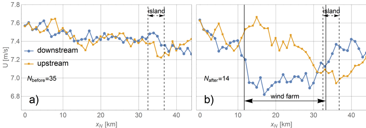
Figure 8: Wind speed transects from a) before and b) after wind farm construction for wind directions directions between 75° and 105°. East is upstream and West is downstream of the (potential) wind farm location. The position of the wind farm to the East/West and Anholt Island to the East of the transects are indicated.
