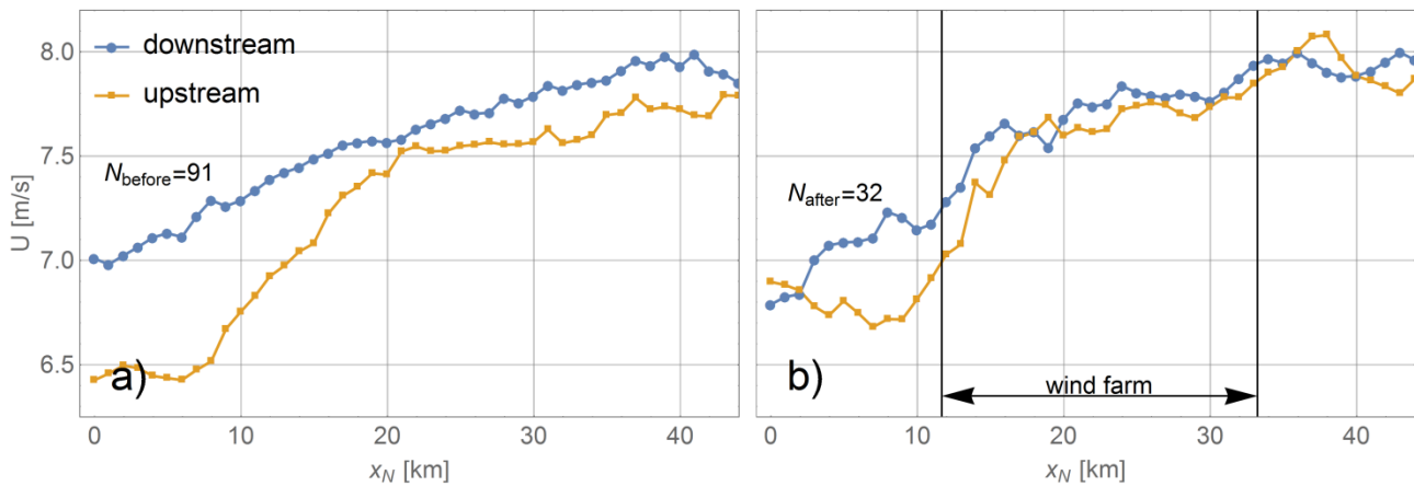
Figure 10: Wind speed transects similar Figure 8 from a) before and b) after construction for wind direction between 255° and 285°. Transect West is upstream and East is downstream of the (potential) wind farm location.
