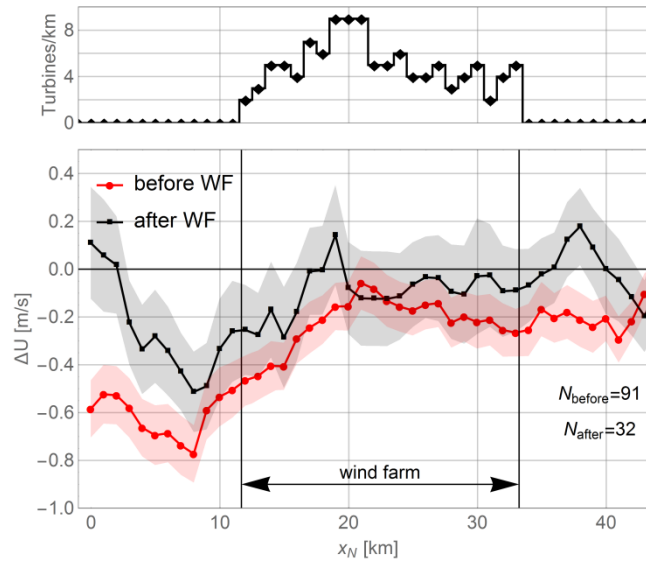
Figure 11: Wind speed difference similar to Figure 9 for short fetch situations with wind directions between 255^\circ and 285^\circ .
