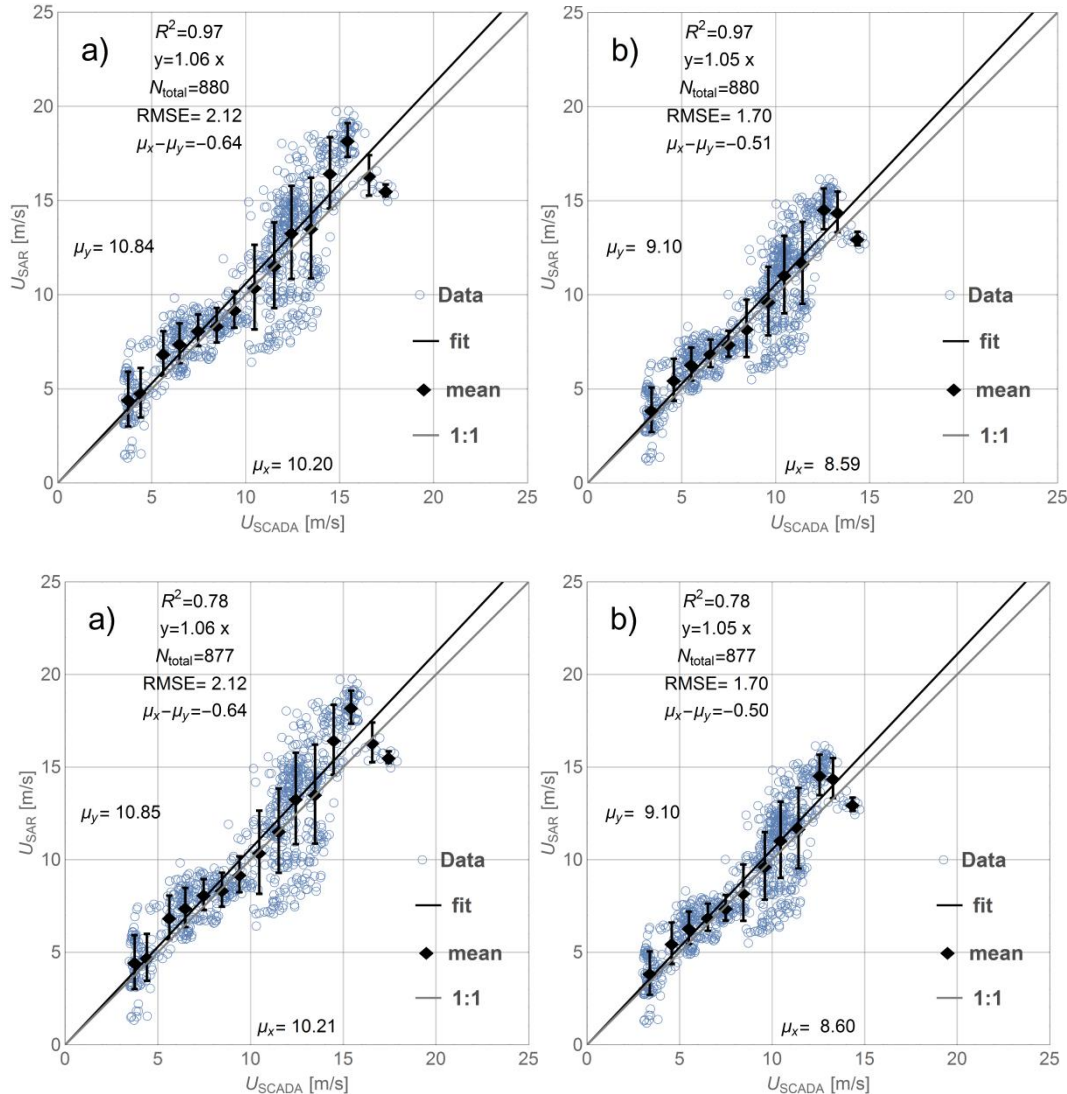
Figure 5: Comparison between SCADA derived wind speeds ( U_{SCADA} ) and SAR derived wind speed ( U_{SAR} ) downstream of the wind turbines: a) for the turbine hub height (81.6 m), b) for the reference height 10 m.
