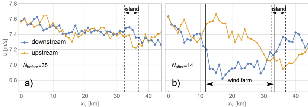
Figure 8: Wind speed transects from a) before and b) after wind farm construction for wind directions between 75° and 105°. East is upstream and West is downstream of the (potential) wind farm location. The position of the wind farm to the East/West and Anholt Island to the East of the transects are indicated.
