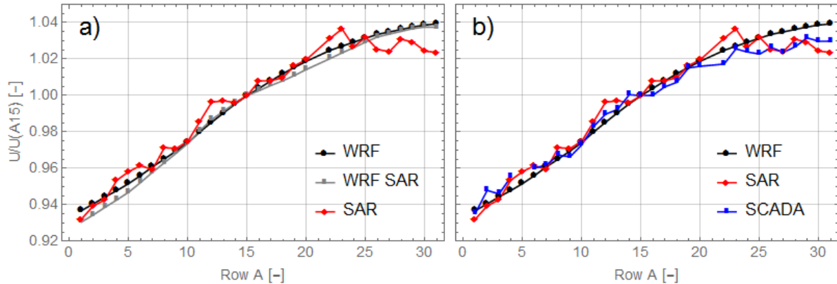
Figure 6: Average wind speed relative to turbine A15 for wind directions between 245° and 275°. a) Data from WRF (2002-2012) and SAR (2002-2012). The entire time period is used for “WRF” and WRF data coinciding with SAR images are used in “WRF SAR”. b) Data from full WRF time series, SAR, and SCADA (2013-2015). No turbine was erected at location A21.
