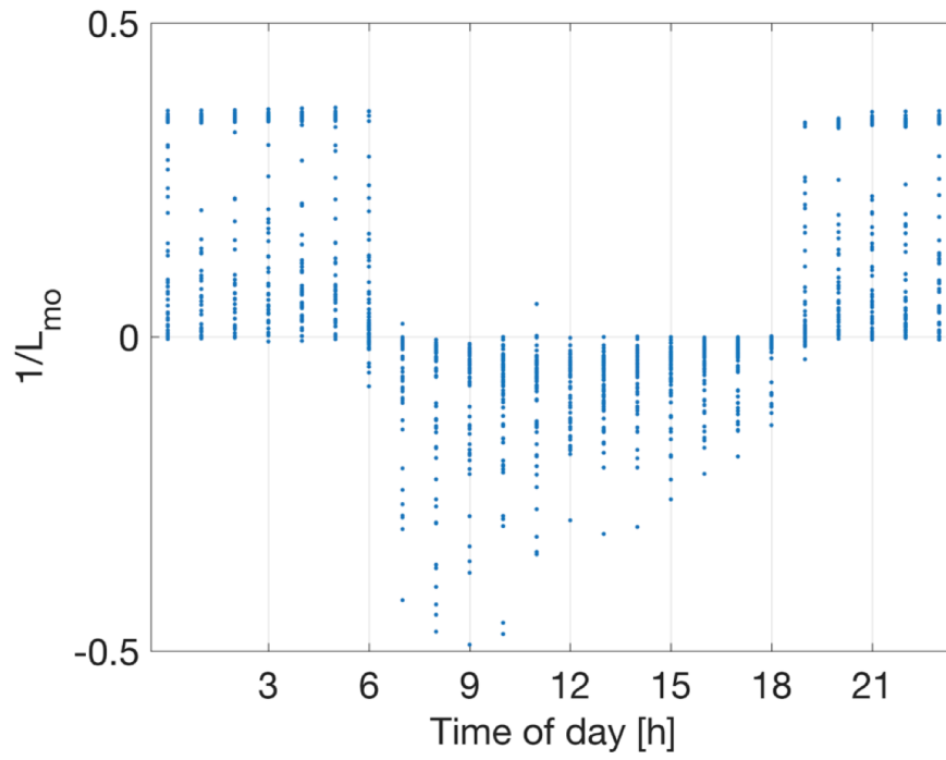
Fig. 1. Diurnal cycle of the Obukhov length for the period of the measurement campaign.
