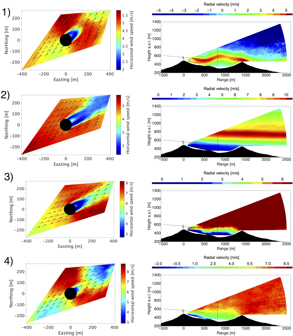
Figure 9. Observed wake cases with the diamond scan (left) and transect scan (right). 1) downwards displaced wake, stable atmospheric conditions + atmospheric wave, 2) no displacement, stable atmospheric conditions, 3) no displacement, neutral atmospheric conditions 4) upwards displaced wake, unstable atmospheric conditions. (measurements of example periods taken: 1) 02:52 – 03:02 UTC 9 June 2015, 2) 06:18 – 06:28 UTC 7 June 2015, 3) 22:20 – 22:30 UTC 10 June 2015, 4) 11:16 – 11:26 UTC 10 June 2015 )
