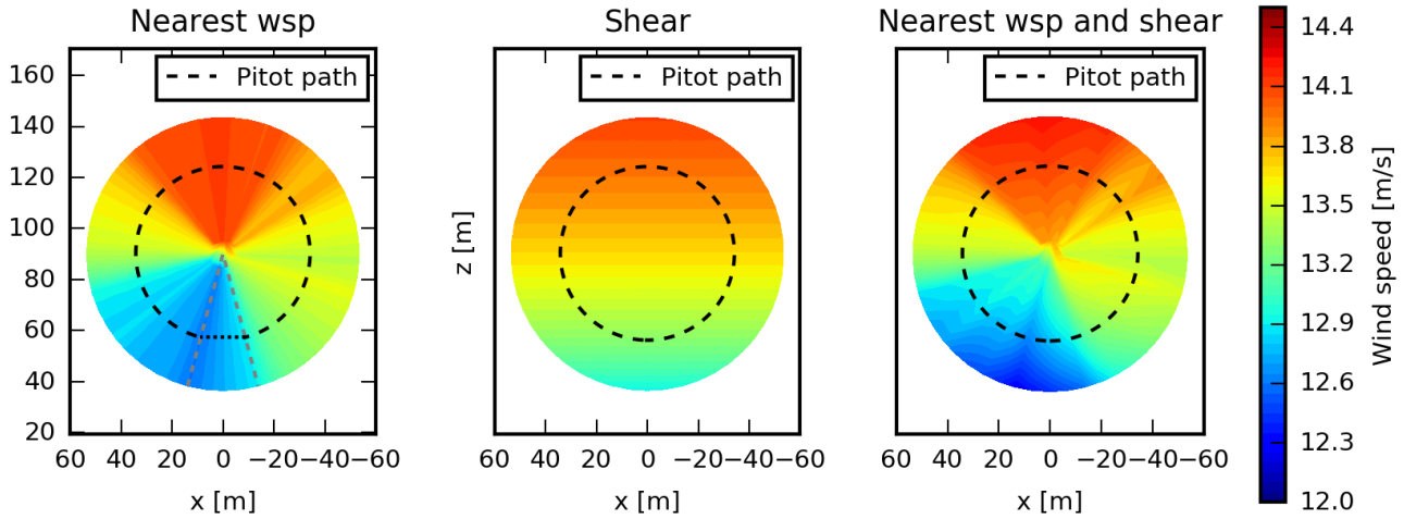
Figure 6. Left: wind speed based on nearest pitot-tube wind speed (interpolated values are used in a 30° sector around the tower to exclude effects of tower shadow). Middle: wind speed based on the one-hour power-shear profile. Right: wind speed based on the nearest pitot-tube wind speed and power shear profile.
