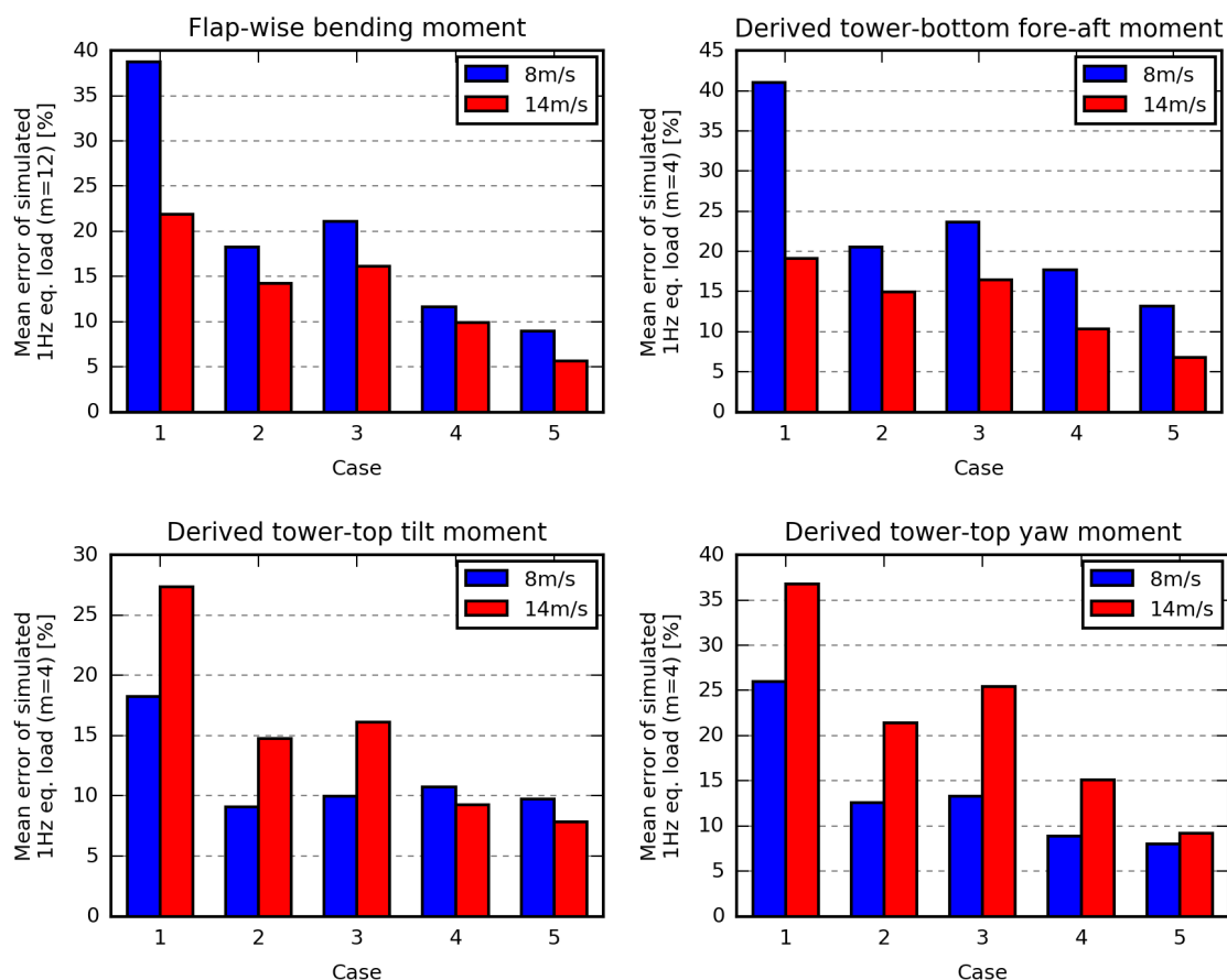
Figure 10. Mean absolute error of the simulated equivalent loads.
