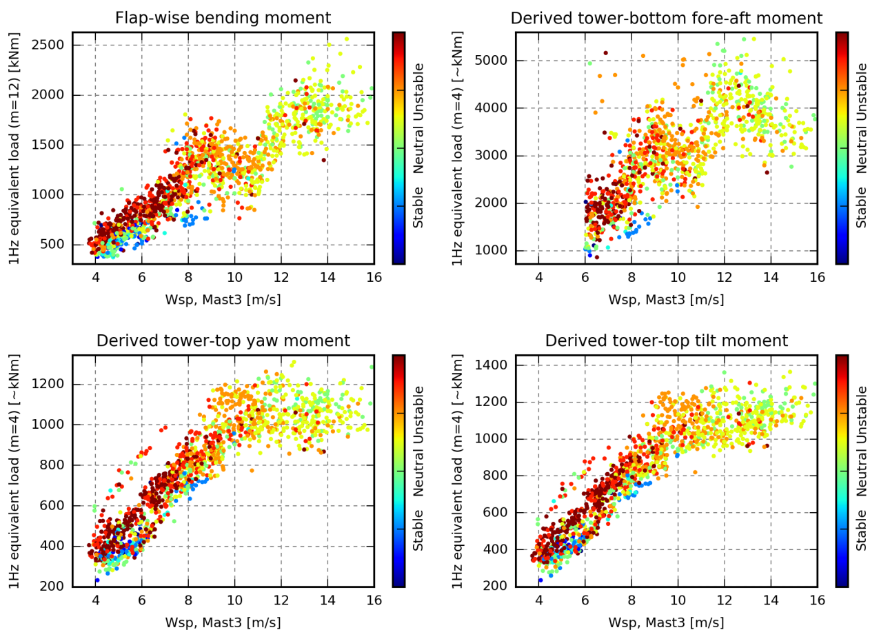
Figure 9. 1 Hz equivalent loads coloured by atmospheric stability extracted from the main met mast.
