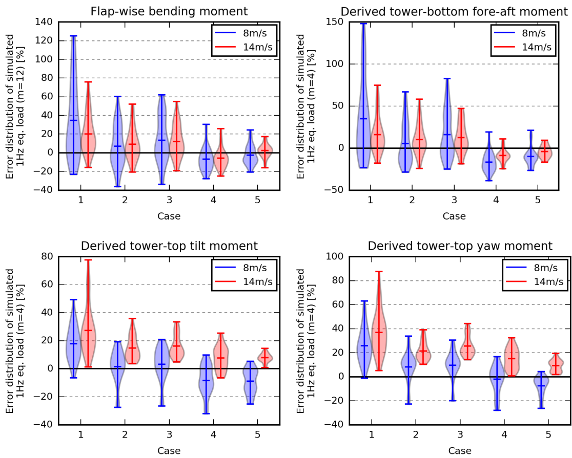
Figure 11. Error distribution of the simulated equivalent loads.
