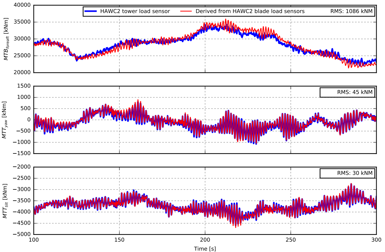
Figure 4. Comparison of the HAWC2 simulated tower loads and the derived tower loads, which is derived from the HAWC2 simulated blade-root load sensors and calibrated for 8 \text{ ms}^{-1} .
